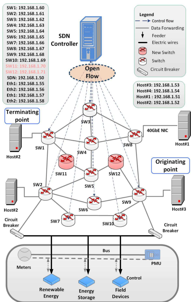
Fig. 5. Network Upgrading Scenario.
