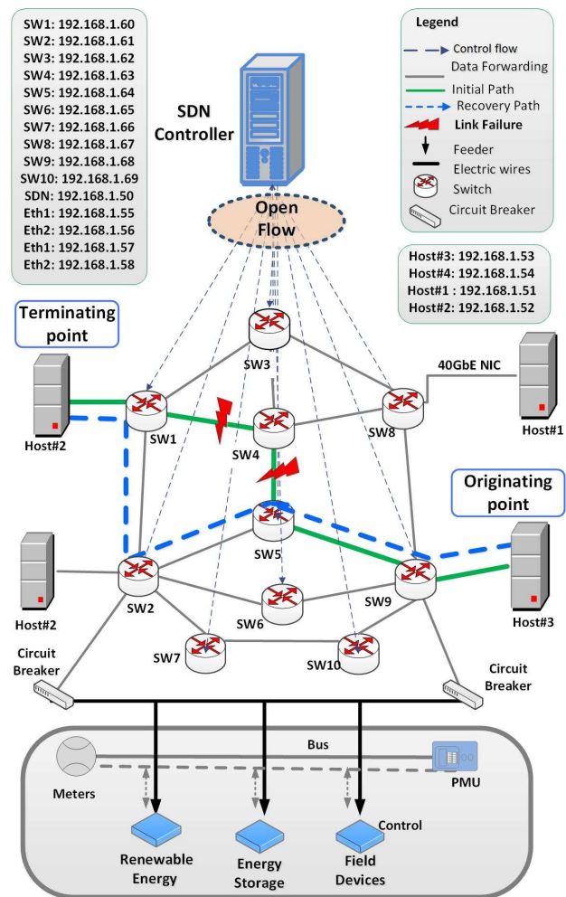
Fig. 4. Network Fault Detection Scenario.
