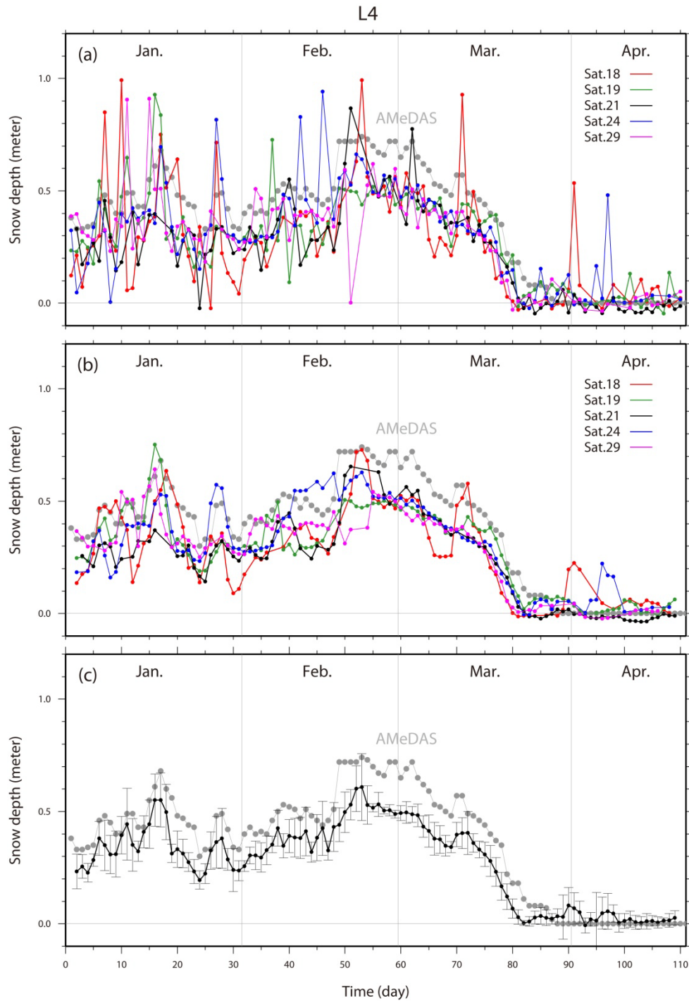
Figure. 7 (a) Raw snow depth time series obtained using L4 data from satellites 18, 19, 21, 24, and 29. The AMeDAS snow depth time series are shown with gray dots. (b) To reduce noise, spectrograms of the three consecutive days have been stacked to estimate the spectral peak of the middle day. (c) Daily averages of the snow depths by the five satellites in (b). The error bars show one standard deviation, and the average standard deviation was \sim 0.062 m. The whole time series is shifted negatively from AMeDAS by \sim 0.1 m.
