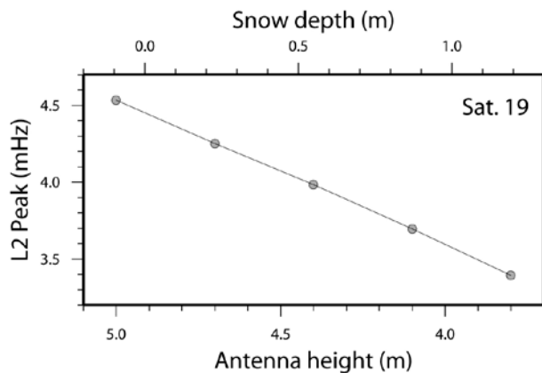
Figure. 3. Calibration curve to relate the L2 peak frequency to the snow depth inferred from synthesized multipath signatures as shown in Fig. 2a. The calibration equation is expressed as [Snow depth] (meter) = \{4.4 - [\text{Frequency peak}] (\text{mHz})\} / 0.93 . This curve is valid only for the ascending satellite 19 received at the Shinshinotsu GPS station.
