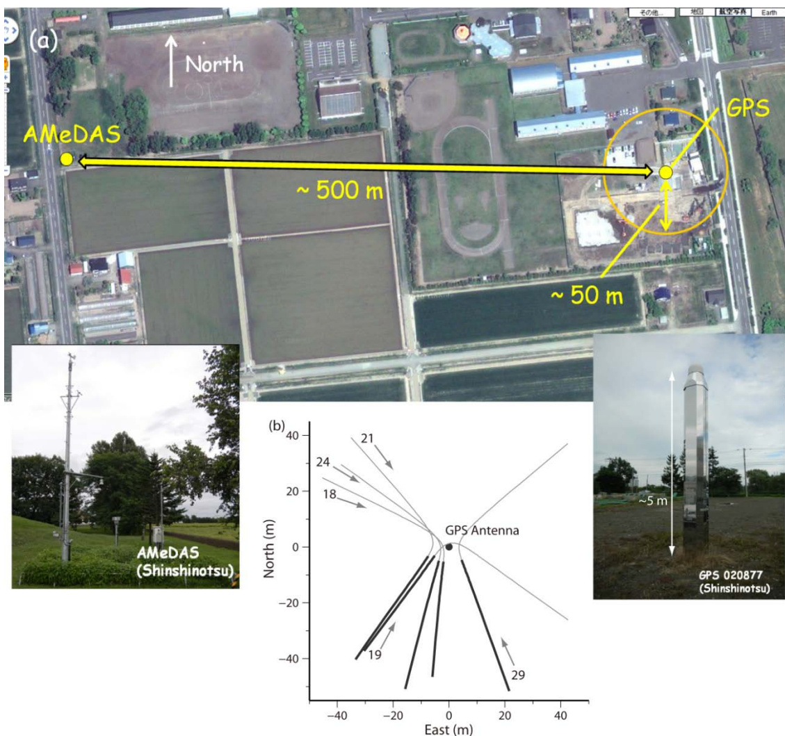
Figure 4. (a) The Shinshinotsu site with a GEONET GPS antenna (right inset), and an AMeDAS snow depth sensor (left inset) \sim 500 m to the west. Ground reflection points responsible for multipath are within \sim 50 m from the antenna (yellow circle). Aerial photograph is from the Google Map. In (b) we show the reflection point trajectories of five GPS satellites analyzed in this study (actual footprints have diameters of a few meters coming from the first Fresnel zone). A black dot indicates the GPS antenna. Thick parts of the curves are used for the analysis of snow depths.
