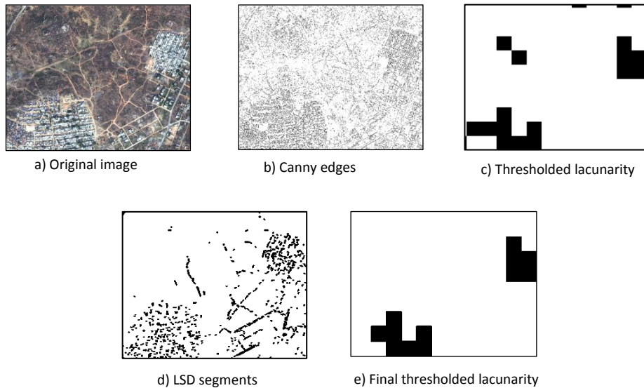
Figure 5. Example of combination of Canny and LSD algorithms for slum identification.
