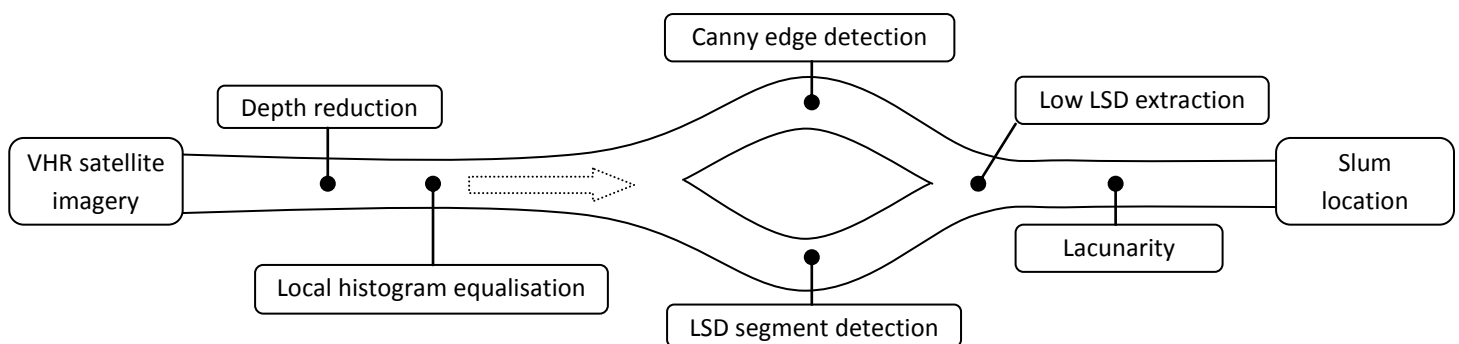
Figure 3. Slum identification algorithm flowchart
