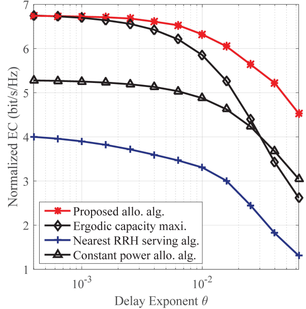
Fig. 5. The sum normalized EC vs delay exponent \theta for our proposed algorithm and the ergodic capacity maximization algorithm, when supporting two users by four RRHs located at [650, 650] , [-650, 650] , [-650, -650] , and [650, -650] .
