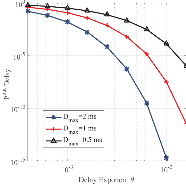
Fig. 3. Delay-outage probability versus delay exponent \theta for various values of D_{\max} for our proposed algorithm.
