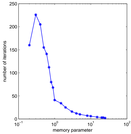
Figure 5.4: The iteration count as m increases: IC(1, 0, m) for the simple Laplace equation
