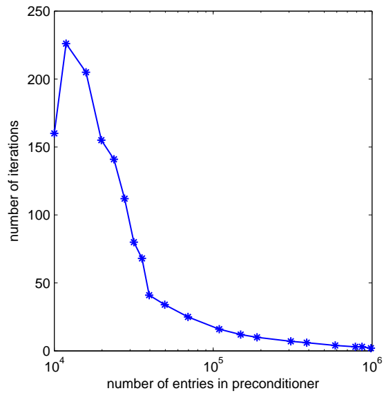
Figure 5.5: The iteration count as nz(\hat{L}) increases: IC(1, 0, m) for the simple Laplace equation
