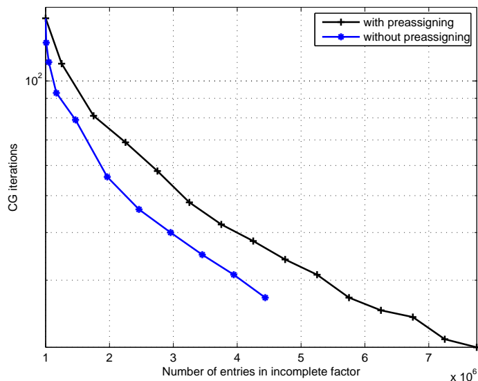
Figure 5.1: The effect of allowing variable levels for problem carsten . Results are given for \ell = 1, \dots, 15 .
