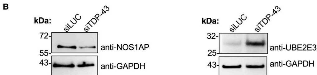
Figure 4 Analysis of seven co-regulated transcripts among TDP-43 and hnRNPs. (A) qPCR validation of C1orf226 , CHPF2 , IGF2 , IRAK2 , RNF112 , NOS1AP and UBE2E3 following TDP-43 knockdown in SH-SY5Y cells. Each bar reports the mean \pm SEM of three independent experiments. Nonparametric un-paired t -test was considered for statistical significance (* P < 0.05 , ** P < 0.01 , *** P < 0.001 ). (B) Western Blotting analysis of NOS1AP and UBE2E3 expression in siTDP-43 treated cells. Expression of GAPDH is also reported as loading control. For each analysis, three independent experiments were performed, and an exemplificative western blot figure was reported.
