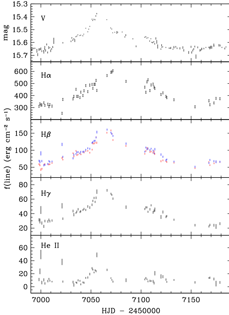
FIG. 1.— Arp 151 light curves for the V -band and the emission lines H\alpha , H\beta , H\gamma , and He\ II as determined from the FLOYDS spectra. The red and blue points show the H\beta light curve determined from the 1st and 2nd order FLOYDS spectra, respectively, as this emission line is visible in both simultaneously. The normalized excess rms scatter of the [OIII] light curve has been added in quadrature to the photon-counting error bars on each data point to take in account of systematic errors.
