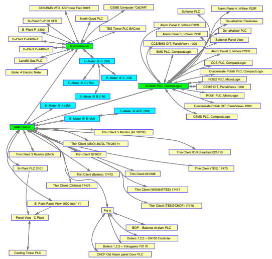
Fig. 3. The PLC and the electrical meter maps
