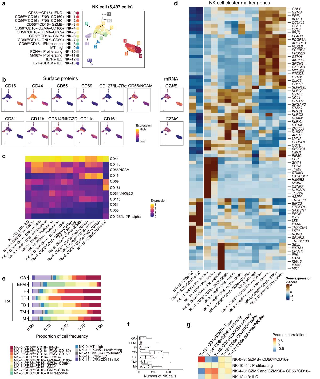
Extended Data Fig. 5 | NK cell-specific analysis. a , NK cell UMAP colored by fine-grained cell state clusters, b , Expression of selected surface proteins or mRNA transcripts among NK cells colored from blue (low) to yellow (high), c , Heatmap of surface protein expression in NK cell clusters colored according to the average normalized expression across cells in the cluster, d , Heatmap of gene expression in NK cell clusters colored according to the average normalized expression across cells in the cluster, scaled for each gene across clusters, e , Distribution of NK cells across clusters, stratified by CTAP. The size
