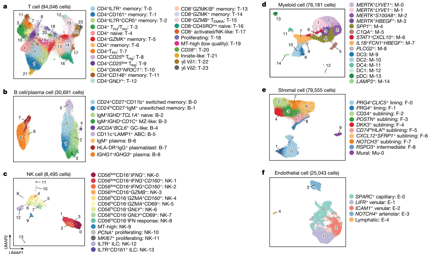
Fig. 2 | Cell-type-specific single-cell analysis captures 77 distinct cell states in rheumatoid arthritis synovium. a–f , Cell-type-specific reference UMAPs for T cells (a) B/plasma cells (b), NK cells (c), myeloid cells (d), stromal cells (e)
