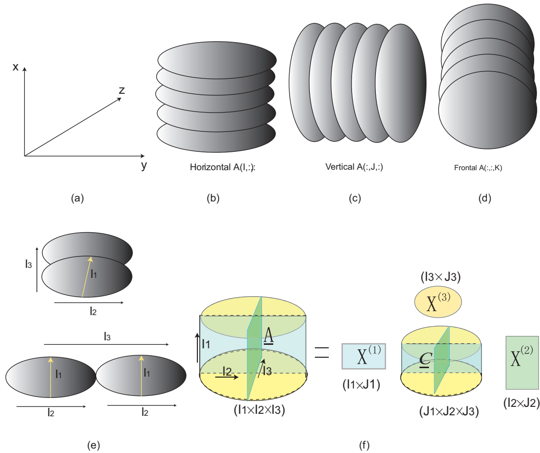
Fig. 15. (a) Illustration of the directions regarding the x -, y -, and z -axis. (b), (c), and (d). Illustration of three direction slices of a third order tensor: horizontal, vertical, and frontal, respectively, which are perpendicular to the x -, y -, and z -axis, respectively. (e) Illustration of the way to flatten the third order tensors along frontal slices. The colon (:) used in the figure indicates all the column elements at a given direction are involved to form an image matrix. (f) Illustration of a third-order decomposition.
