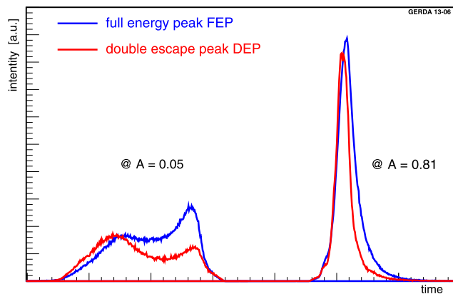
Fig. 14 Time distribution for crossing the 5% (left) and 81% (right) pulse height for ^{228}\text{Th} calibration events with energy close to the DEP (red) and close to the 1621 keV FEP (blue) (Color figure online)
