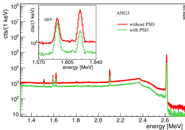
Fig. 17 228 Th calibration spectrum without and with TMIpANN pulse shape discrimination for ANG 3. The PSD cut is fixed to retain 90 % of DEP events (see inset)
