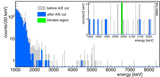
Fig. 11 Energy spectrum of the combined BEGe data set: grey (blue) before (after) the PSD cut. The inset shows a zoom at the region Q_{\beta\beta} \pm 200 keV with the 8 keV blinded region in green (Color figure online)
