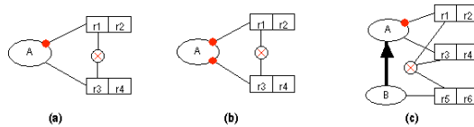
Fig. 4. Unsatisfiable schemes because of mandatory and exclusion conflicts.
