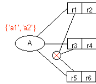
Fig. 7. Contradiction between value and exclusion constraints.
