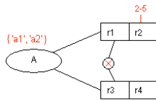
Fig. 6. Contradiction between value, exclusion, and frequency constraints.
