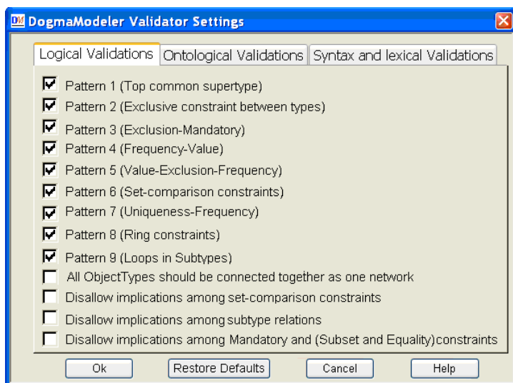
Fig. 15. DogmaModeler's support of logical validations.
