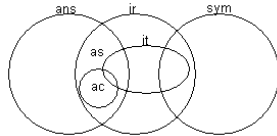
Fig. 12. Relationships between ring constraints [H01].
