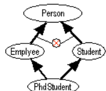
Fig. 1. Unsatisfiability of ORM schema.
