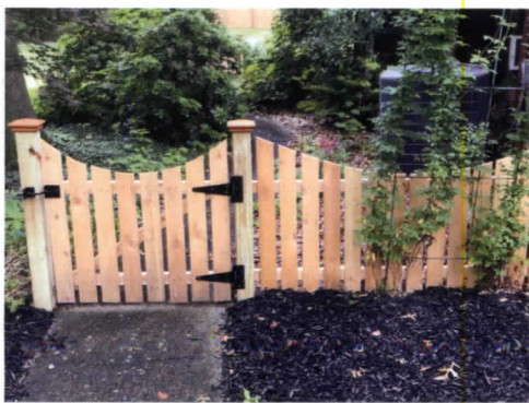
Red cedar, scalloped spaced picket, 4" boards, 1" space, cedar post caps and walk gate
