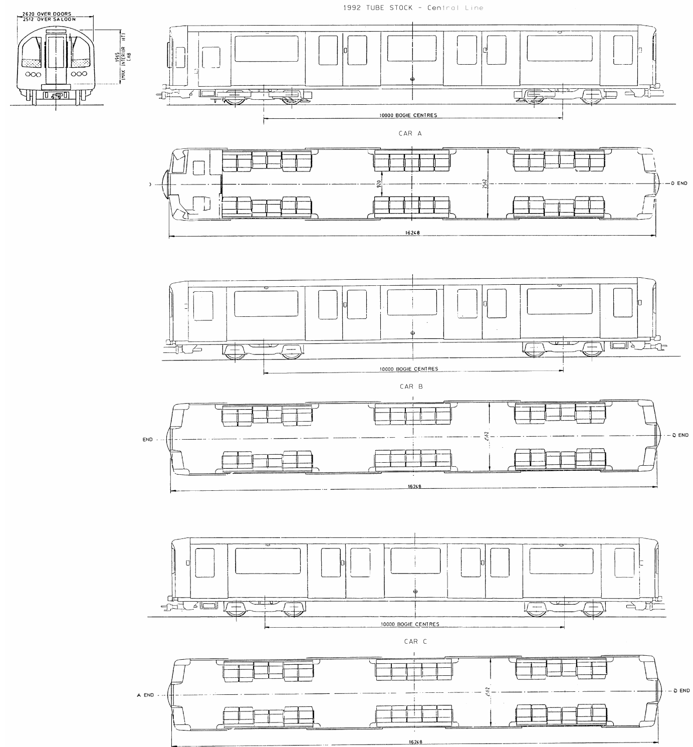
1992 TUBE STOCK (TARE WEIGHT - 170.00 TONNES - 8 CAR TRAIN)
