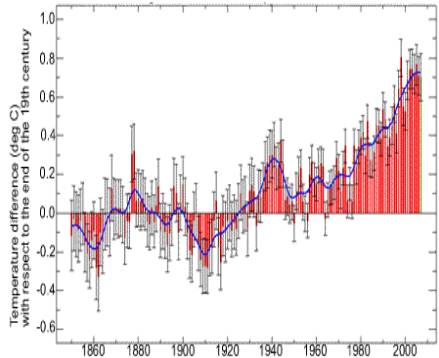
Global temperature, 1850-2007
