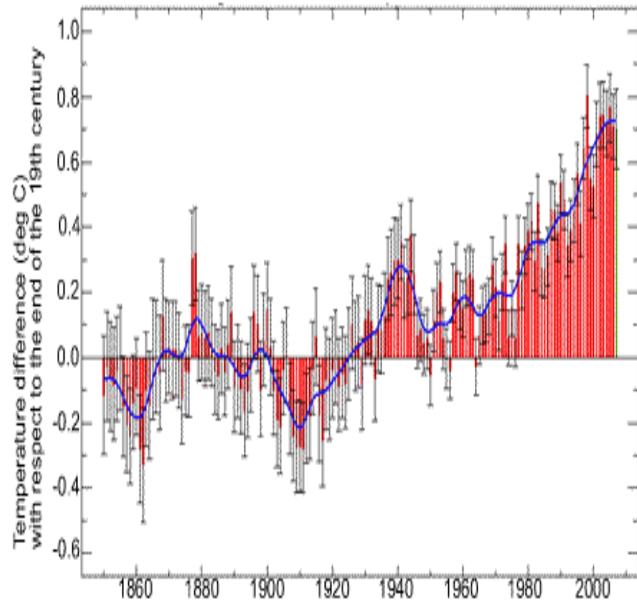
Global temperature, 1850-2007
