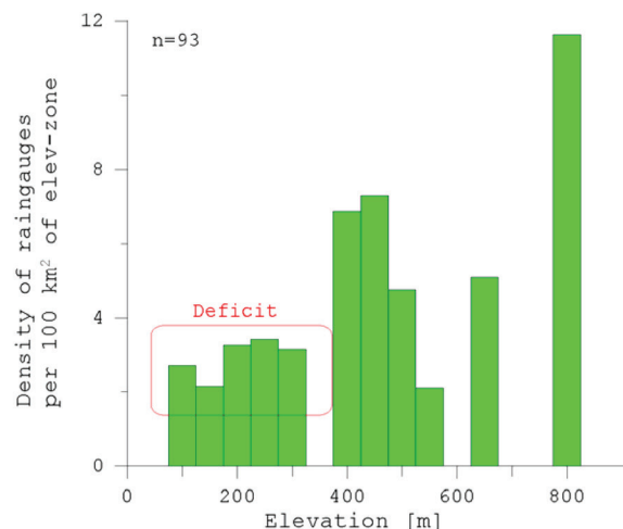
Fig. 5. Degree of completeness of precipitation time series for the Bode River basin and surroundings from 1961 to 2006 (left), and histogram of the density of rain gauges per 100 km 2 of elevation zone within the Bode basin (right).
