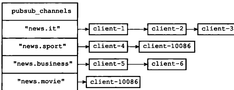
图 18-19 pubsub_channels 字典
