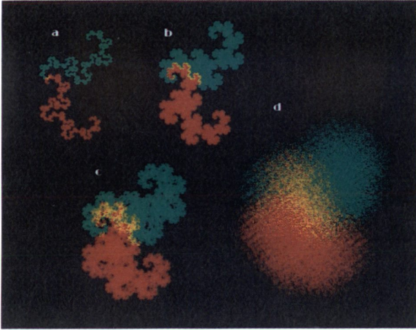
Plate 6.2. Variations of the dragon curve. a) \gamma = 0.65 . b) \gamma = 0.7071 = \sqrt{2}/2 . c) \gamma = 0.75 . d) \gamma = 0.85 .
