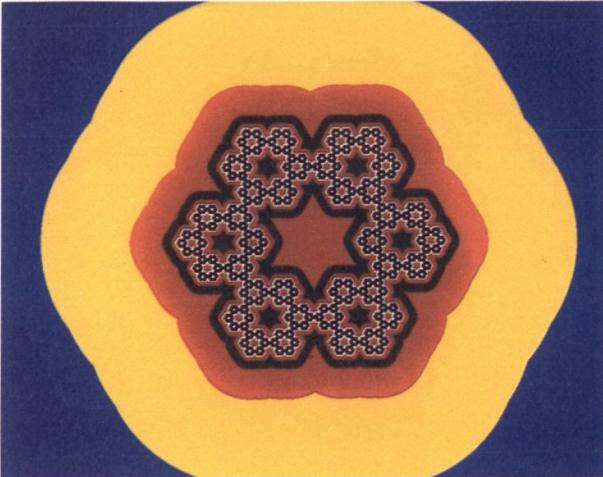
Plate 7.4. The "multi-snowflake" curve generated using the repelling method.
