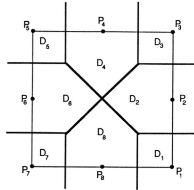
Fig. 7.5. Relative position of the scaling centers P_1 - P_8 and domains D_1 - D_8 for generating the Sierpiński carpet.
