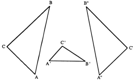
Triangle A'B'C' is related to ABC by a direct similarity Triangle A''B''C'' is not directly similar to ABC because the mapping of ABC to A''B''C'' involves a reflection.
