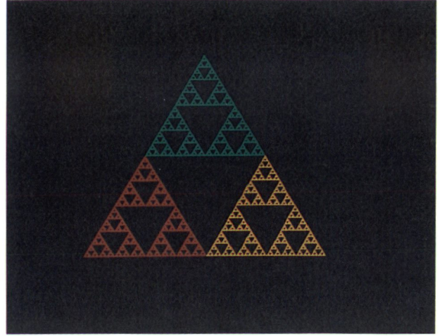
Plate 6.3. The Sierpiński gasket approximated using the attractive method.
