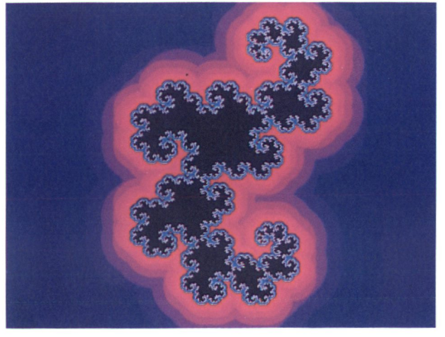
Plate 7.9. The dragon curve generated using the repelling method.
