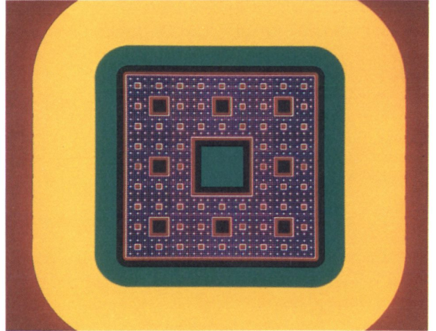
Plate 7.6. The Sierpiński carpet generated using the repelling method.
