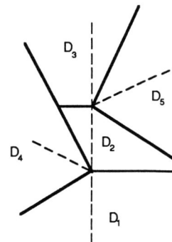
Fig. 7.7. Partition of the plane into domains D_1 - D_5 for generating a twig using the repelling method.
