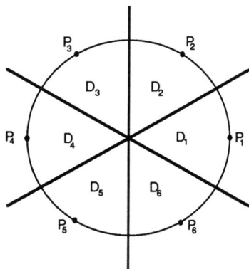
Fig. 7.3. Relative position of the scaling centers P_1 - P_6 and domains D_1 - D_6 for generating the "multi-snowflake" of Plate 7.4. All scaling ratios are equal to 3.
