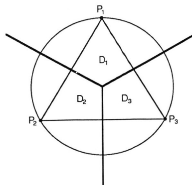
Fig. 7.1. Relative position of the scaling centers P_1 - P_3 and domains D_1 - D_3 for generating the Sierpiński gasket using the repelling method. All scaling ratios are equal to 2.
