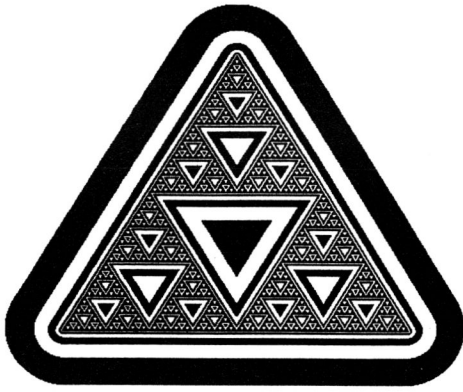
Fig. 7.2. The Sierpiński gasket generated using the repelling method.
