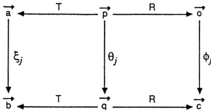
Fig. 2.2. Relationship between mappings \theta_j , \phi_j , \xi_j , R and T .
