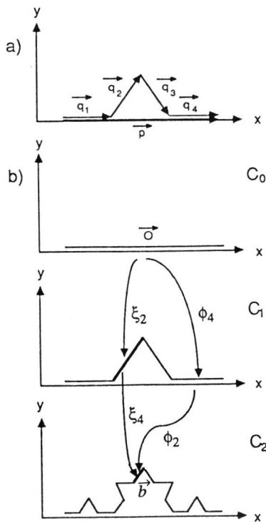
Fig. 3.1. a) The production of a Koch system. b) Two methods for obtaining a vector \vec{b} \in C_2 : a sequence of productions and a sequence of similarities.
