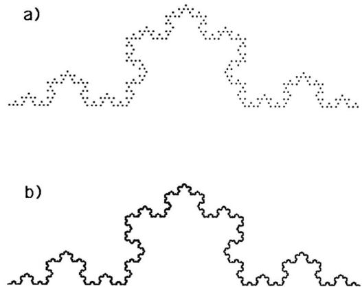
Fig. 6.1. Two approximations of the limit snowflake curve obtained by the attractive method. Approximation (a) consists of 100 points. Approximation (b) has 10,000 points.
