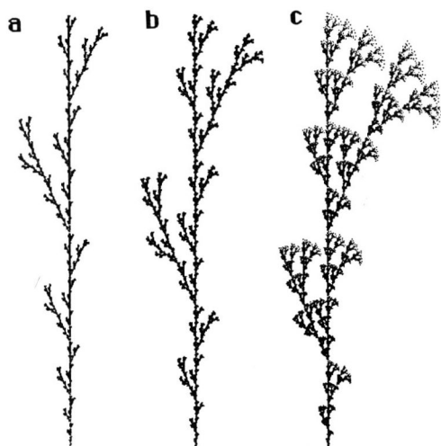
Fig 6.5. "Twigs" generated using the attractive method.
