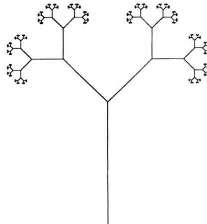
Fig. 8.1. An example nonuniform fractal generated using the attractive method.
