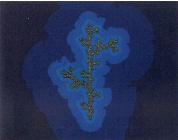
Plate 7.8. A "twig" generated using the repelling method.
