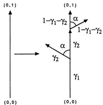
Fig. 6.4. Production of the Koch system generating twig-like shapes.
