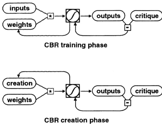
Fig. 1. A simplified schematic of Creation by Refinement using a gradient descent learning procedure such as Back Propagation.
