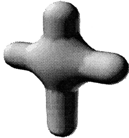
Figure 7: A blend of two cylinders using an order zero continuous Bernstein-Bézier blending function with four control points.
