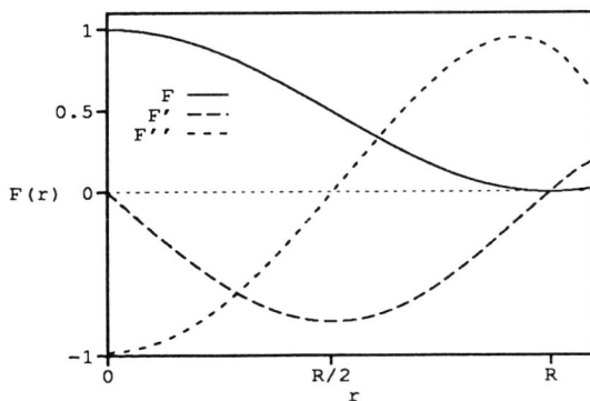
Figure 5: Cubic blending function and its derivatives. ( F' = 0.5 \frac{dF}{dr} , F'' = 0.2 \frac{d^2F}{dr^2} )
