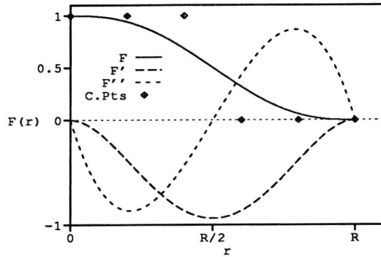
Figure 6: Fifth degree Bernstein-Bézier blending function, its control points and derivatives. ( F' = 0.5 \frac{dF}{dr} , F'' = 0.15 \frac{d^2F}{dr^2} ) Note that both derivatives have zero values at the end points.
