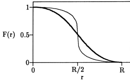
Figure 11: Single segment cubic Bézier blending functions (parametric). The four control points are (0, 1) , (c, 1) , (R-c, 0) , (1, 0) , where 1/3 < c < 1 . The soft (thick) curve is identical to the cubic curve F_{cub} .
