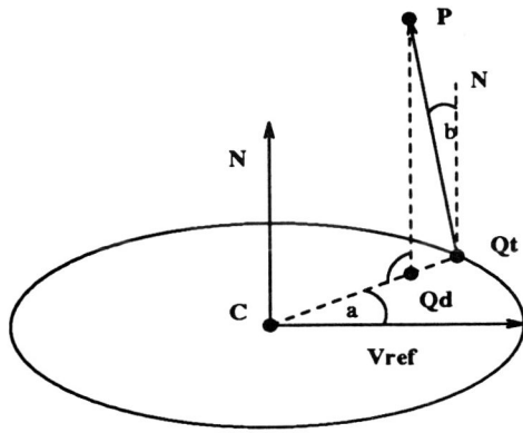
Figure 13: Parameters that can be used to modify the blending function of a circle or torus ( \alpha = a, \beta = b ).
