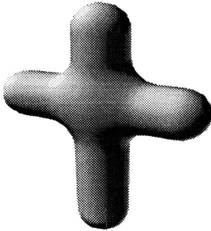
Figure 9: A blend of two cylinders using a second order continuous Bernstein-Bézier blending function with six control points (Figure 6).
