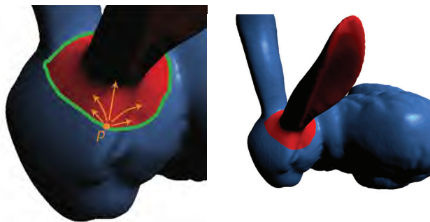
Figure 6: Flood-filling determines the “interior” of the selection. Left: The detail shows the boundary C on the surface shaded green, the marked subset of the surface shaded red. The orange arrows show the direction of flood-filling from the selection point p on the boundary towards the interior of the closed curve \hat{C} in screen space. Right: The object viewed at large.
