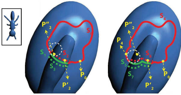
Figure 16: Occlusion-aware region extension by the example of brush painting. Left: Frame i - 1 : The brush is outlined in white. \hat{C}^{i-1} projects to segments S_{0,3} (only S_0 and S_1 are visible). Assume the selected region is bounded by S_0 \cup S_2 . Right: Frame i : P_0 and P'_2 project back to both \hat{C}^i and \hat{C}^{i-1} , therefore tracing from either will get the intended region, which is bounded by S_4 \cup S_6 . P''_2 and P_4 , on the other hand, do not satisfy the condition.
