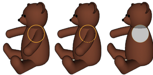
Figure 2: Occlusion-aware surface cut from 2D curve in screen space. A 2D curve is projected onto the surface in a closed curve. Thanks to occlusion-awareness the cut-out is performed on the body, removing the arm entirely, instead of a "cookie-cut" (simple removal of surface points mapping back inside/onto 2D curve).
