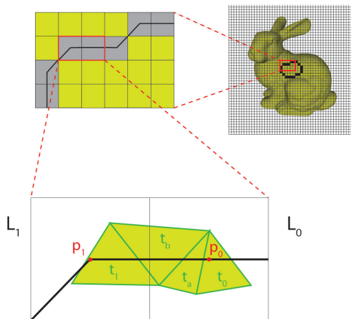
Figure 8: Finding curves on a mesh. Upper right: Discrete user input in screen space (thinned to a 4-connected curve) on the BUNNY model. Upper left: Detail of input (shaded grey). Bottom: Detail of two pixels on the curve. The triangle index of the visible fragment at the center of each pixel is stored ( t_0 for L_0 and t_1 for L_1 ). Assume the tracing starts at pixel L_0 to find C . The projection of [p_0, p_1] intersects triangles t_0, t_a, t_b , and t_2 , and they are all added to C . The process continues with [p_1, p_2] and subsequent line segments, until C is completed when t_0 is reached in L_0 again.
