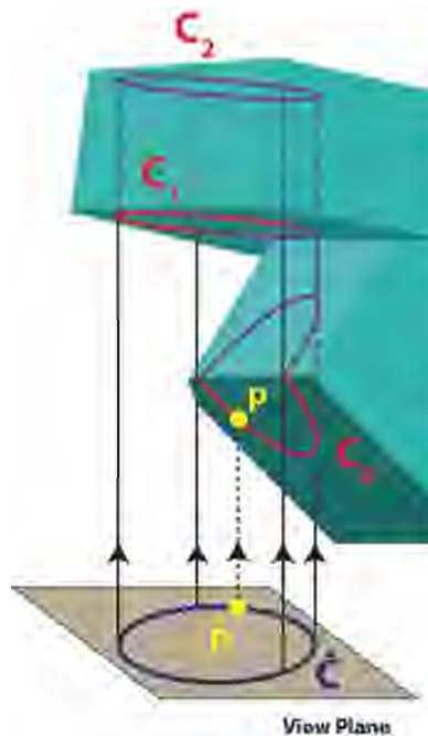
Figure 4: The blue curve \hat{C} drawn on the view plane is projected onto the model surface as a number of curves C_{0..2} . The curve segments are colored red (visible), or magenta (occluded). \mathbb{C} = \{C_0, C_1, C_2\} , while the candidate set is \mathbb{C}_{vis} = \{C_0, C_1\} , as C_2 is entirely invisible. \hat{p} on \hat{C} is the selection point , and p is its closest projection onto the surface. In the figure, p lies on C_0 , so C = C_0 is the boundary curve selected.
