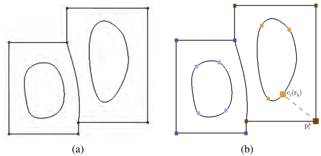
Figure 7: Segmenting two adjacent cells: (a) Corners are detected along the cell boundary; (b) Corresponding curve points are found on the cell curve. These points are connected to form the 4-sided regions required for Coons patch creation.
