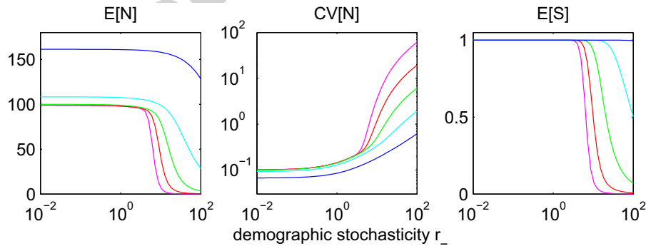
Figure 2: Population properties as functions of model parameters. Left: mean population size \mathbb{E}[N] . Middle: coefficient of variation of population size CV[N] . Right: expected number of species \mathbb{E}[S] . The demographic stochasticity coefficient r_- is plotted on the x -axis; the curves are parametrized by the immigration rate \mu : 0.01 (magenta), 0.1 (red), 1 (green), 10 (cyan), 100 (blue).
