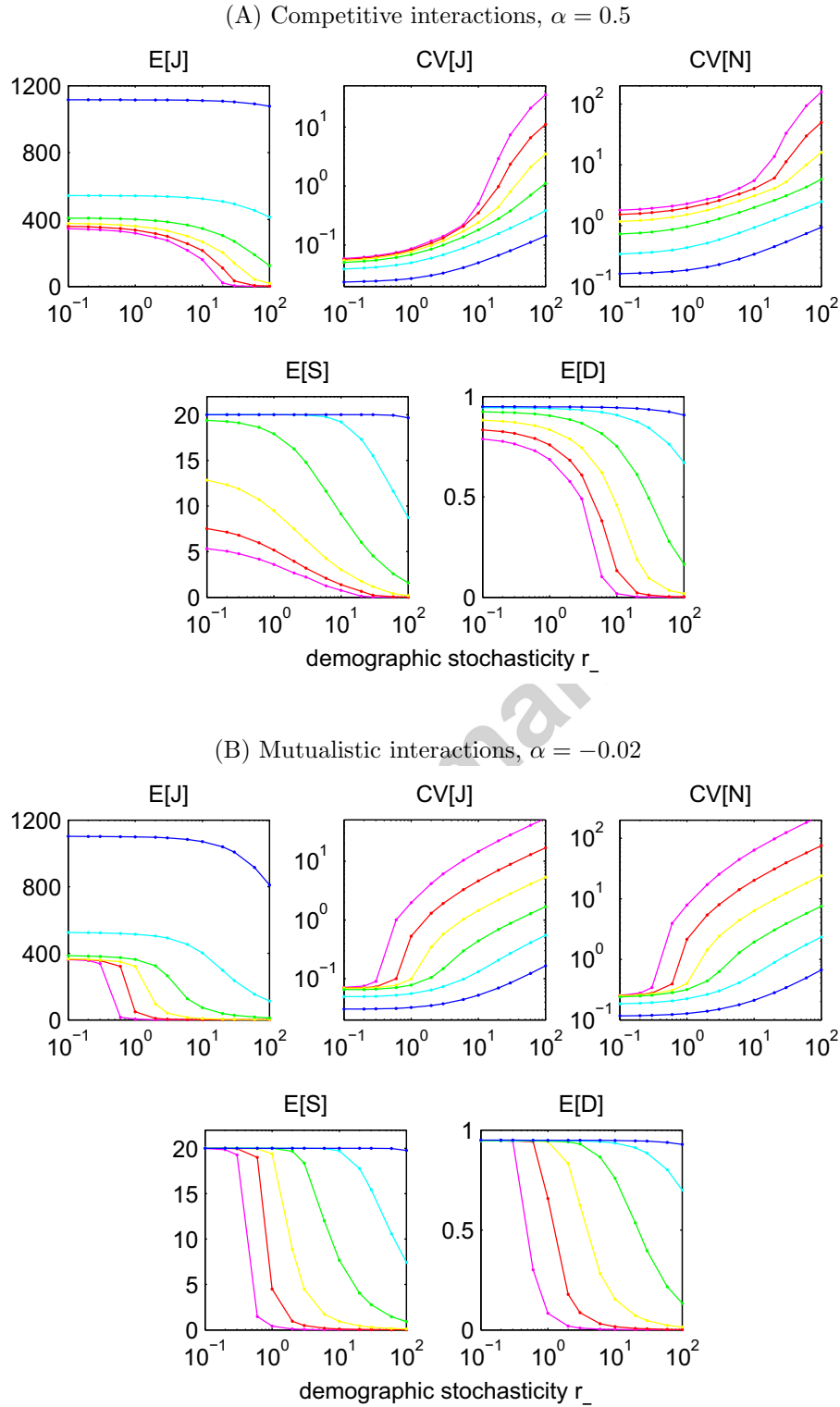
Figure 5: Community properties as functions of demographic stochasticity coefficient r_ for different immigration rates \mu . The immigration rate varies from 0.001 to 100 with the same color code as in Figure 3. The interaction coefficient \alpha takes two different values: (A) \alpha = 0.5 , (B) \alpha = -0.02 . The community carrying capacity K is constant, K = 400 .
