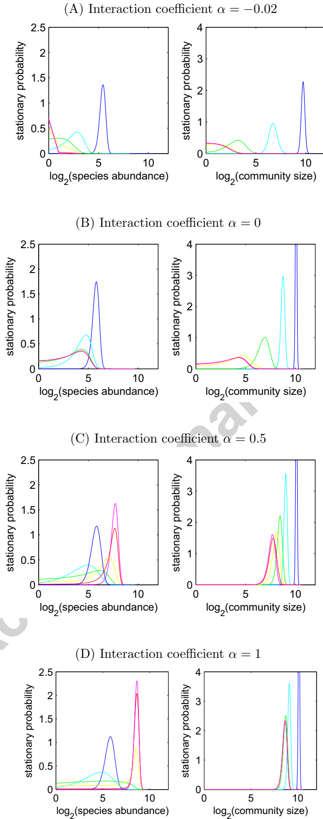
Figure 3: Species abundance and community size distributions as functions of interaction coefficient \alpha and immigration rate \mu . The immigration rate \mu takes values 0.001 (magenta), 0.01 (red), 0.1 (yellow), 1 (green), 10 (cyan), and 100 (blue). The demographic stochasticity coefficient r_- is the same for all distributions, r_- = 10 . The interaction coefficient \alpha takes four different values: (A) \alpha = -0.02 ; (B) \alpha = 0 ; (C) \alpha = 0.5 ; (D) \alpha = 1 . The community carrying capacity K is constant, K = 400 .
