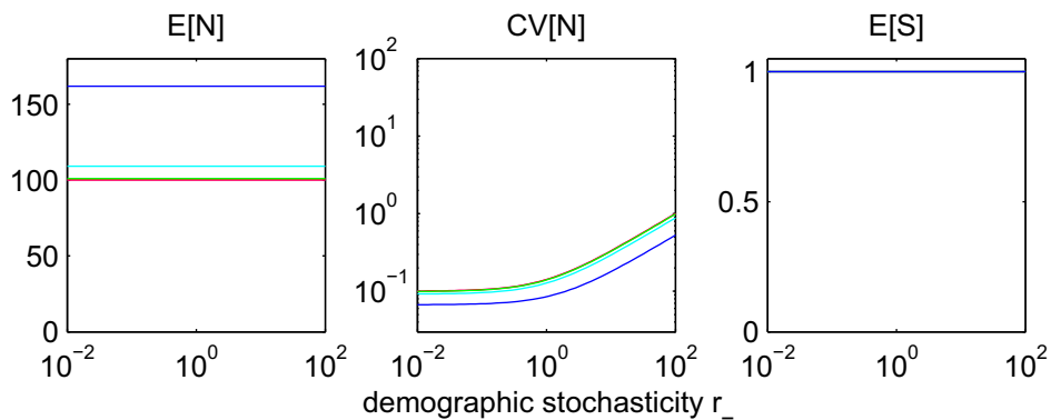
Figure S2: Same as Figure 2, but for linear approximation.
