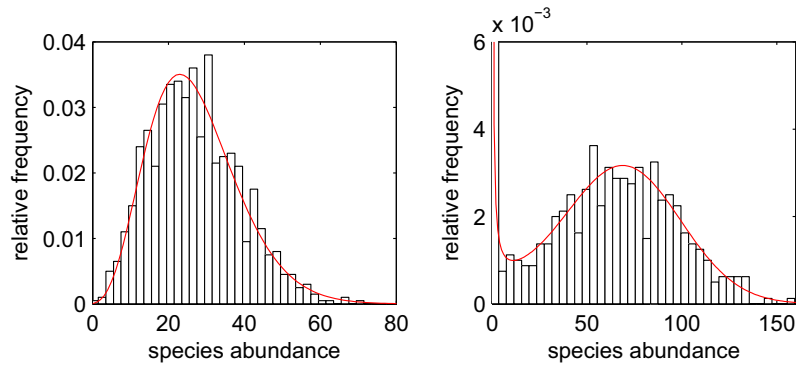
Figure S1: Comparison between simulated and computed stationary species abundance distribution. The histograms give the species abundance distribution of a simulated trajectory. The model was simulated during 2 \cdot 10^4 time units. The first half was used to eliminate the transient dynamics; the second half was used to sample the population size every 10 time units (1000 samples in total). The red curves correspond to the approximation (E6). Parameters are r_- = 1 , \alpha = 0.5 , K = 400 . Left panel: \mu = 10 . Right panel: \mu = 0.01 .
