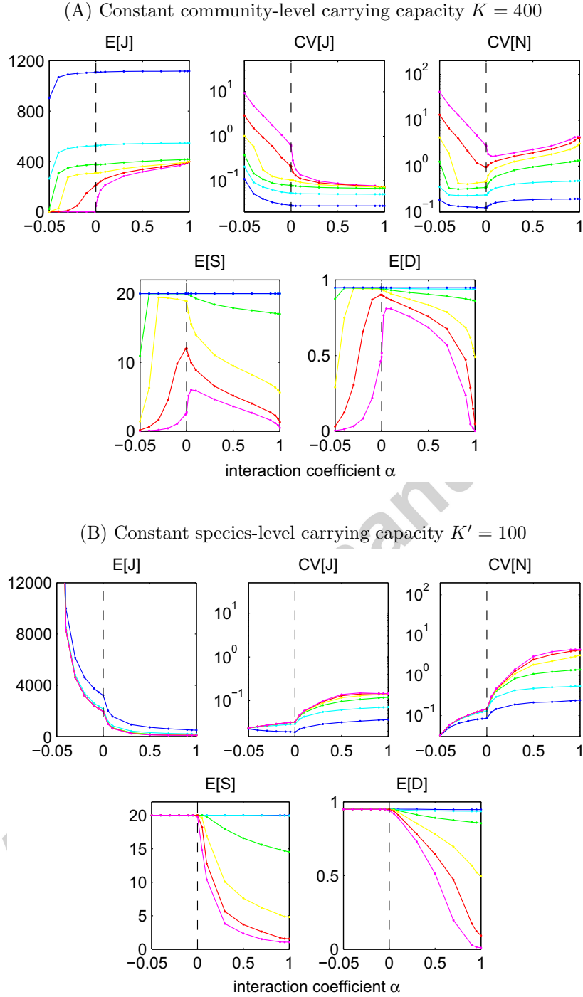
Figure 4: Community properties as functions of interaction coefficient \alpha for different immigration rates \mu . The immigration rate varies from 0.001 to 100 with the same color code as in Figure 3. The demographic stochasticity coefficient r_- is the same for all curves: r_- = 1 . The scale for mutualistic interactions ( \alpha < 0 ) is ten times finer than the scale for competitive interactions ( \alpha > 0 ). In part (A) the community-level carrying capacity K is constant, K = 400 ; in part (B) the species-level carrying capacity K' is constant, K' = 100 .
