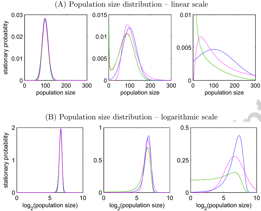
Figure 1: Comparison of stationary population size distribution for different stochastic models and their approximations. In red: density-dependent mortality (6); in green: density-dependent natality (7); in blue: linear approximation (B4); in magenta: linear approximation (B5). Left: r_- = 1 ; middle: r_- = 10 ; right: r_- = 100 . Other parameters are K = 100 , \mu = 0.1 , r = 1.0 , r_+ = r + r_- , r'_- = r_+ , r'_+ = r + r'_- .
