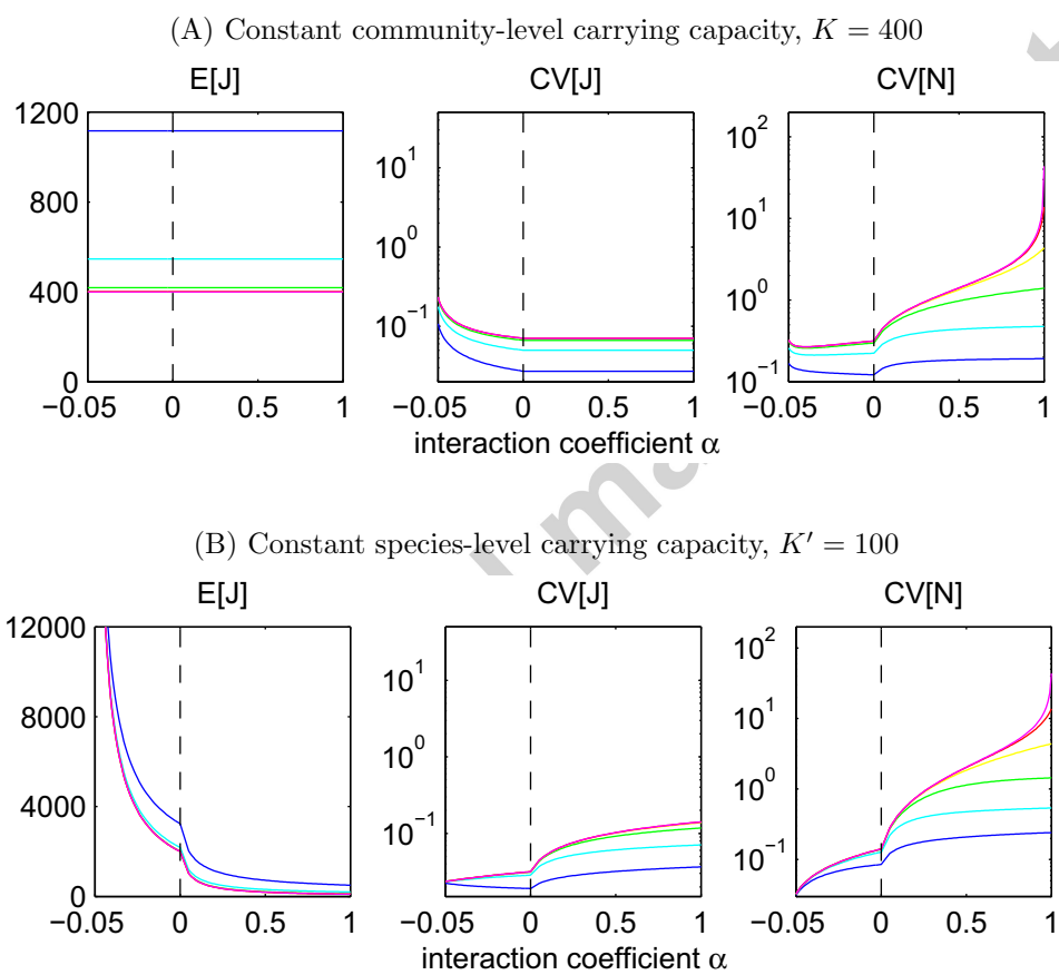
Figure S3: Same as Figure 4, but for linear approximation.
