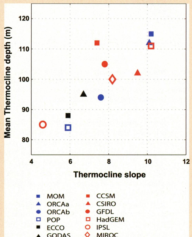
FIG. 2. Mean depth of the equatorial thermocline and mean thermocline slope along the equator as simulated in a number of ocean-only models (blue), data assimilation models (black), and coupled models (red). The thermocline slope is defined as the normalized difference between thermocline depth at 180° and 100°W, where an appropriate isopycnal surface was chosen for each individual model. The thermocline depth corresponds to maximum vertical density gradient along the equator. Note the large differences in the mean thermocline depth and, especially, thermocline slope in the models. After Brown and Fedorov (2008).
