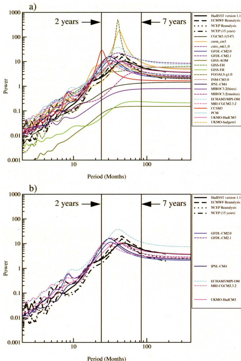
FIG. 3. Niño-3 SST anomaly spectra for IPCC AR4 models in preindustrial conditions. (a) Original figure from AchutaRao and Sperber (2006); (b) “eye-ball” selection of six closest to observed (note that MRI is the only flux-adjusted of the six).
