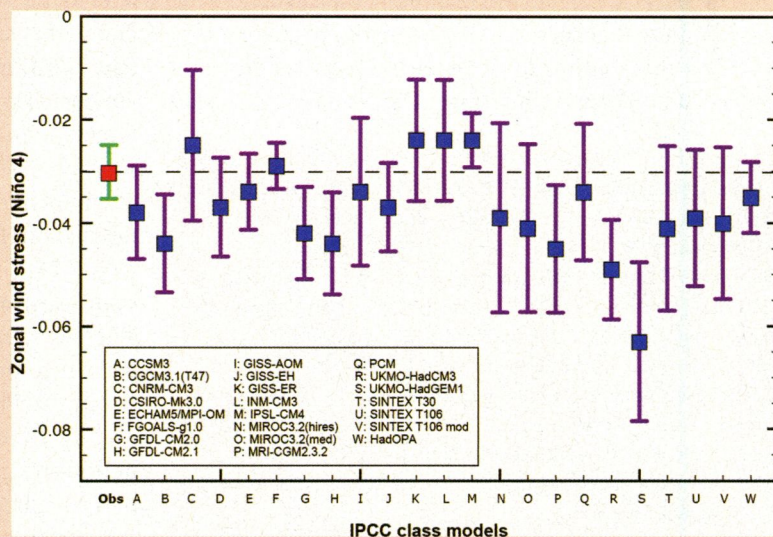
FIG. 1. Mean zonal wind stress (squares) and annual cycle amplitude (bars) in the central-western Pacific (Niño-4 region; see Fig. 4) for the 20th-century simulations of the IPCC AR4. (left) Observations are taken from the 40-yr European Centre for Medium-Range Weather Forecasts (ECWMF) Re-Analysis (ERA40) [1950–2000 average is -0.03 \text{ N m}^{-2} ]. Units are \text{N m}^{-2} .
