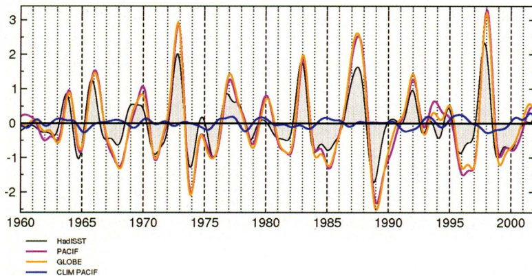
FIG. 7. Evolution of the Niño-3.4 (170°W–110°W, 5°N–5°S) interannual SST anomaly for the HadISST1.1 observations (black), a simulation in which the tropical ERA-40 wind stress has been nudged into the CNRM-CM3 IPCC coupled model (pink), a similar simulation with a global nudging of the wind stress (orange) and a simulation with imposed ERA-40 climatology (blue). After Joly and Voldoire (2009).
