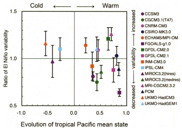
Fig. 6. Mean state change in average tropical Pacific SSTs and change in El Niño variability simulated by AOGCMs (adapted from Meehl et al. 2007b). The mean state change (horizontal axis) is computed over the area 10°S to 10°N, 120°E to 80°W (reproduced from Yamaguchi and Noda 2006). The change in El Niño variability (vertical axis) is denoted by the ratio of the ENSO amplitude between the current climate and the last 50 yr of the SRES A2 experiments (2051–2100), except for FGOALS-g1.0 and MIROC3.2(hires), for which the SRES A1B was used, and UKMO-HadGEM1, for which the 1% yr -1 CO 2 increase climate change experiment was used, in the region 30°S to 30°N, 30°E to 60°W (reproduced from van Oldenborgh et al. 2005). Error bars indicate the 95% confidence interval.
