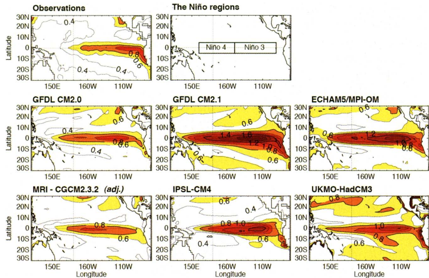
FIG. 4. SST std dev ( ^{\circ}\text{C} ) for 100 yr of monthly data for models in Fig. 3b. Observations are taken from HadISST1.1 (1900–99). The location of the Niño regions discussed in the text is also shown.
