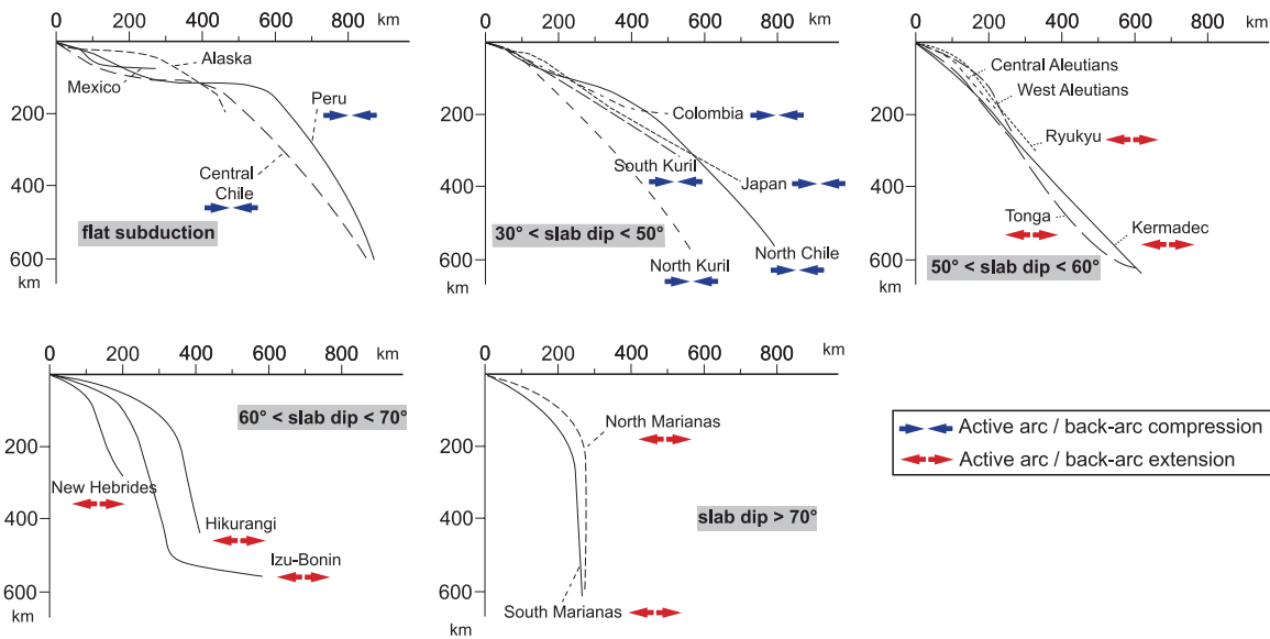
Figure 1. Major Pacific slab geometries classified by groups of deep slab dips except the first group, which concerns flat subductions with variable deep slab dips: 30^\circ to 50^\circ , 50^\circ to 60^\circ , 60^\circ to 70^\circ , steeper than 70^\circ . Active arc/back-arc compression is observed for slab dips lower than 50^\circ , whereas active arc/back-arc extension occurs only for slabs dips steeper than 50^\circ .
