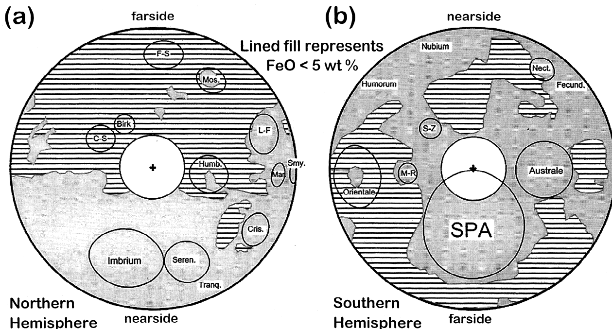
Figure 2. Polar projections of the lunar surface showing regions containing < 5\text{ wt } \% \text{ FeO} as areas with lined fill: (a) northern hemisphere and (b) southern hemisphere. Approximate locations of major impact basins are outlined for reference. The large proportion of area in the northern hemisphere that has \text{FeO} < 5\text{ wt } \% reflects the concentration there of the FHT highly anorthositic central region. In the northern hemisphere, regions that have > 5\text{ wt } \% \text{ FeO} are associated mostly with the PKT. In the southern hemisphere, however, \text{FeO} -rich regions are also associated with SPA and in extensive regions associated with poorly defined, ancient basins such as Australe and possibly some extensive regions of cryptomare in the nearside southern hemisphere. Data are not shown for latitudes 75^\circ to the poles. \text{FeO} was derived from Clementine UVVIS [Lucey et al. , 1998a]. Abbreviations: C-S, Coulomb-Sartung; F-S, Freundlich-Sharanov; L-F, Lomonosov-Fleming; M-R, Mendel-Rydburg; S-Z, Schiller-Zucchius.
