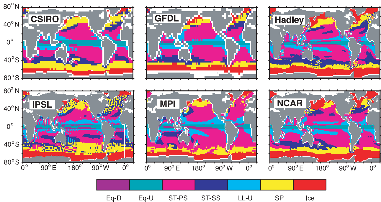
Figure 3. Biome classifications as determined from the AOGCM control climate variables for each of the six models. The color scheme and symbols are described in the Figure 2 caption.
