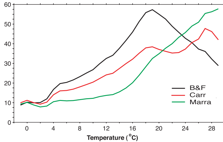
b. Primary Production from data ( \text{g-C m}^{-2} \text{d}^{-1} )
