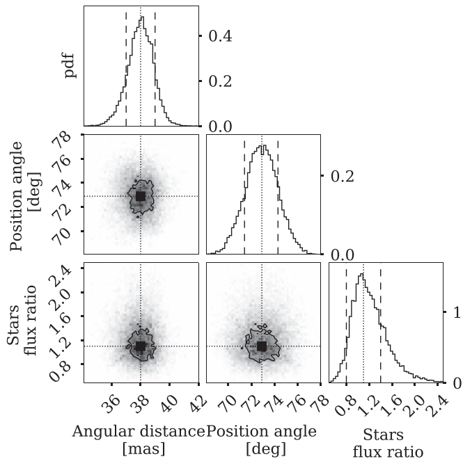
Figure 11. Posterior pdf for the separation, position angle of the secondary with respect to the primary, and the flux ratio of secondary over the primary for the favored model \mathcal{M}_5 . Diagonal panels: marginalized posterior pdf for angular separation of the stars, position angle of the secondary with respect to the primary. The nominal values are indicated by the dotted vertical lines while the dashed vertical lines are the 68% credible intervals. The three remaining panels in the bottom left are the joint posterior pdf for the same parameters. The contours in the joint pdfs are the 39.3% credible intervals.
