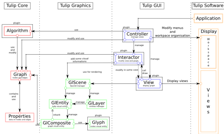
Fig. 2. TULIP architecture overview. The TULIP framework consists of four packages. TULIP core provides an efficient data structures for relational data. TULIP graphics is a complete OpenGL rendering engine. TULIP GUI is a collection of widgets built on top of Qt library for the purpose of information visualization. Finally, TULIP software is an application for embedding algorithms, visualization techniques/interaction, and complete information visualization systems. All these packages can be dynamically extended through the plugin architecture of TULIP.
