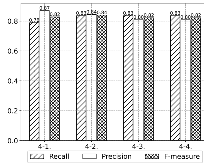
Fig. 7. Experimental results for evaluation item 4 regarding Case 1, 2-3. Qualitative pitch interval, 3-2. Three, and 5-1. Narmour's method (N = 6)
