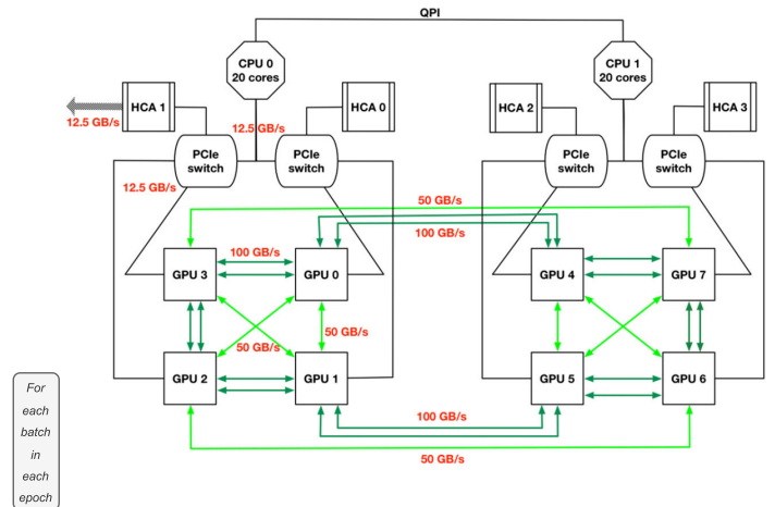
Fig. 7. The DGX-1 Tesla V100 architecture [1], composed of two NUMA (Non-Uniform Memory Access) nodes of 20 cores and 4 GPUs each. GPUs are linked together by the NVLink interconnect (green rows) which ensures an important bandwidth
