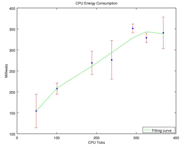
Fig. 17. Power consumption for CPU usage (with standard deviation).
