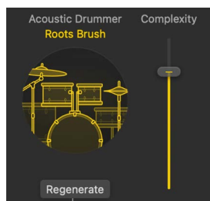
Regenerate button
