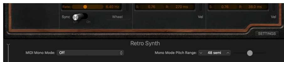
Disclosure arrow
