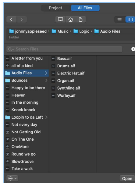
Column View
