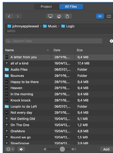
List View
