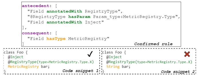
Fig. 6: Encoded rule with correct and incorrect usage.
