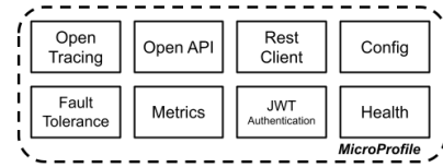
Fig. 1: MicroProfile APIs/components
