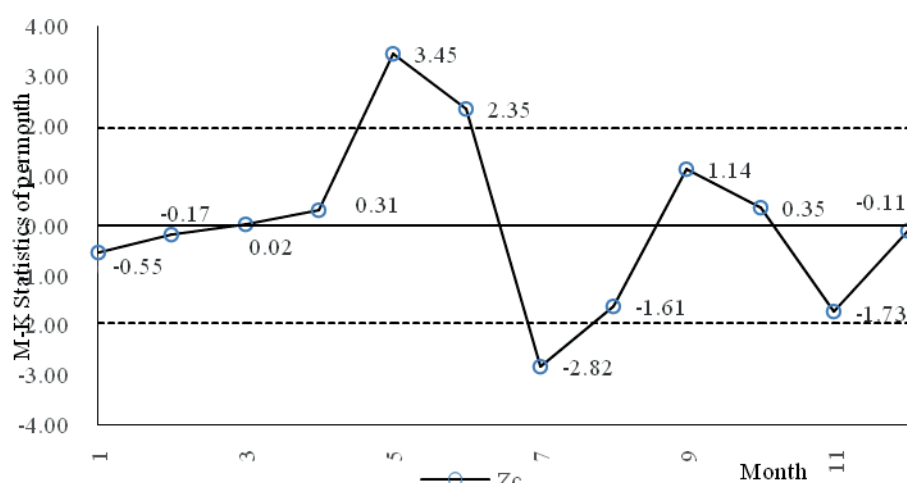
Fig. 3 M-K test of the proportion of the monthly precipitation in Haihe River basin.
