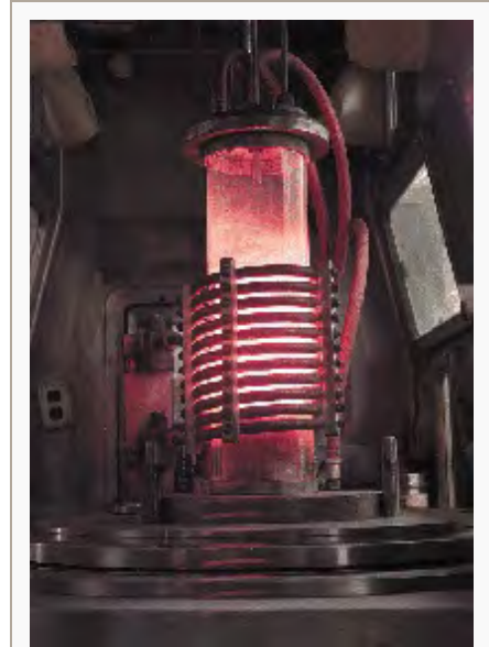
A casting furnace in operation
