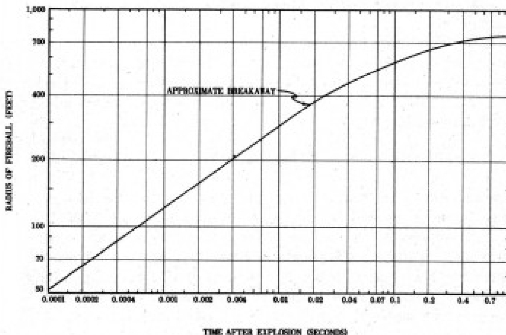
Figure 2.85. Variation of radius of luminous ball of fire with time in a 20-kiloton explosion.
