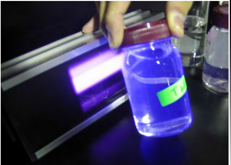
'Cerenkov Radiation'
