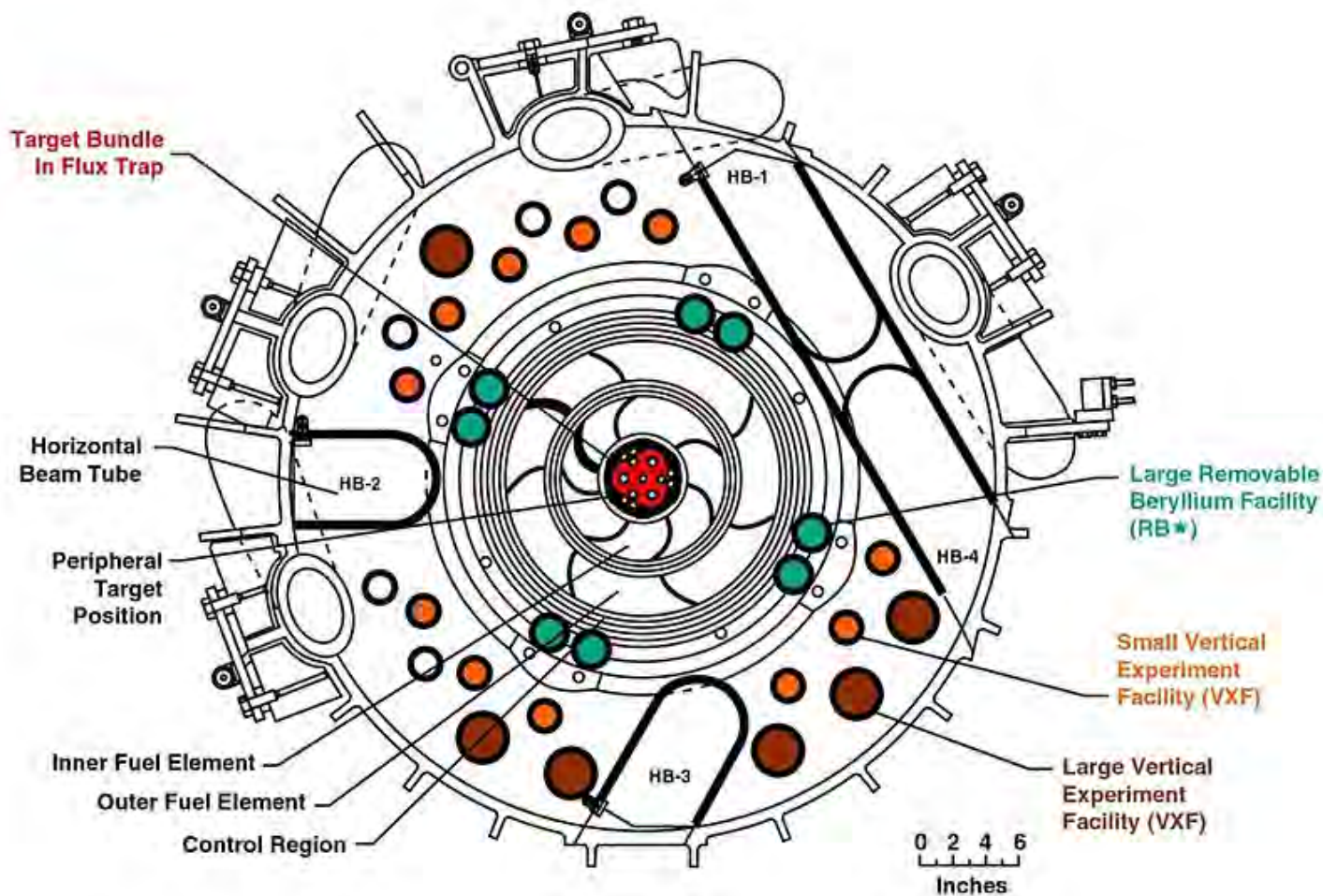
High Flux Isotope Reactor Core – Cross Section
