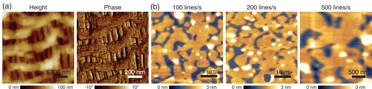
FIG. 7. (a) Imaging of Celgard in air using our AFM head with a FastScan A cantilever at 10 Hz line-rate on a MultiMode AFM with JV scanner and Nanoscope V controller. (b) High-speed tapping mode height images of DLPC/DPPC lipid bilayers at 100–500 Hz line-rate using our AFM head with small cantilevers in fluid, on-line compensation of the lateral scanner dynamics and a high-speed AFM controller.
