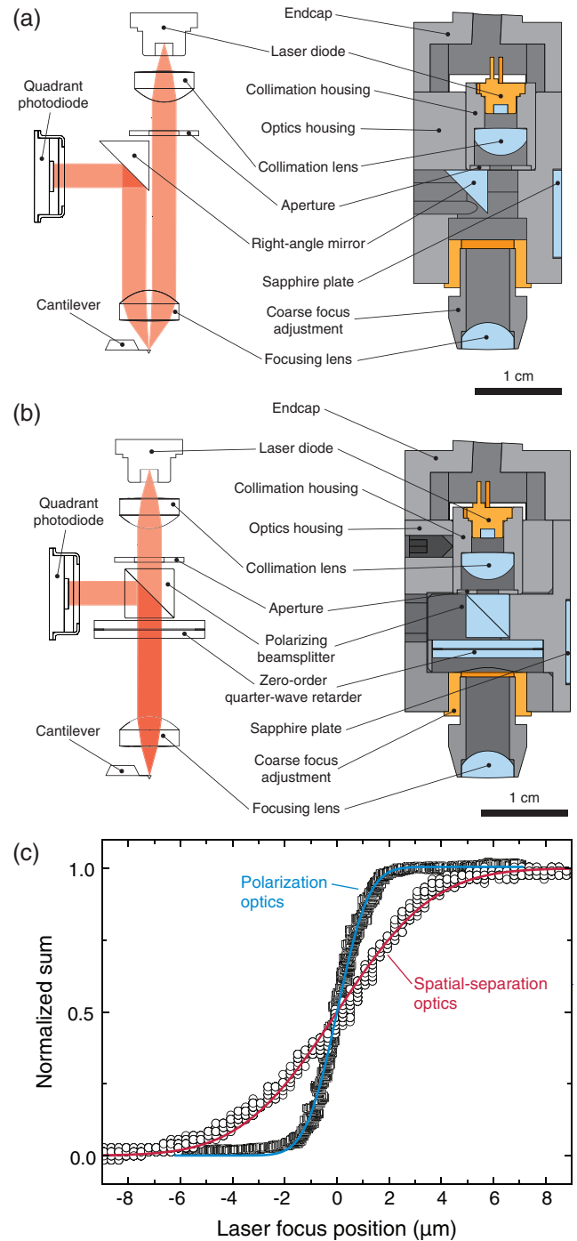
FIG. 2. Schematic of the spatial separation (a) and polarization-based (b) optical beam deflection approaches. The major optical components along with the approximate light paths are shown in isolation on the left, and the mechanical layouts of the components in the two OBD assemblies are shown on the right. (c) Measurement of the focal spot size using a knife-edge technique. The 1/e^2 waist of the spatial separation and polarization-based separation approaches are 5.8 and 1.9 \mu\text{m} , respectively.
