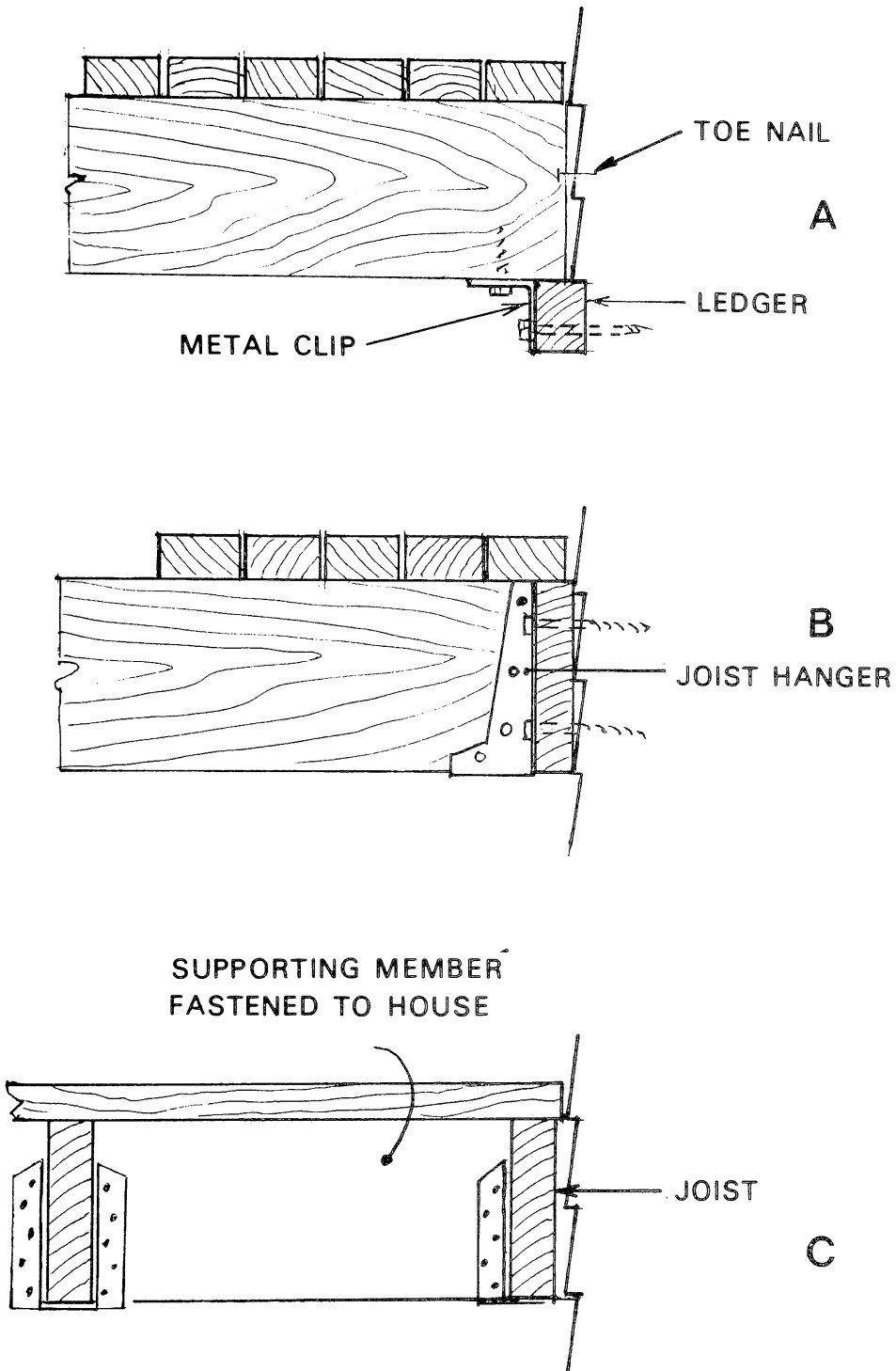
Figure 28. — Joist to house. A — ledger support; B — joist hangers; C — unconnected joists.
