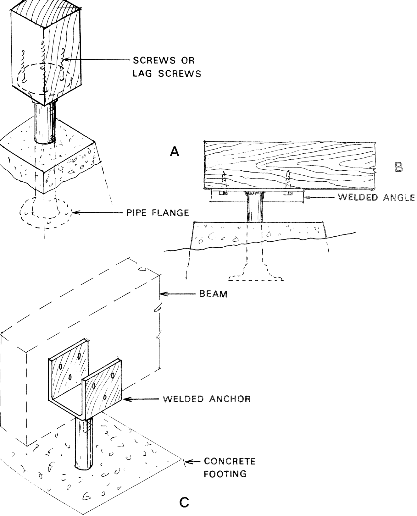
Figure 17. — Pipe and flange anchor. A — pipe flange; B — welded angle (low decks); C — saddle anchor for low decks.
