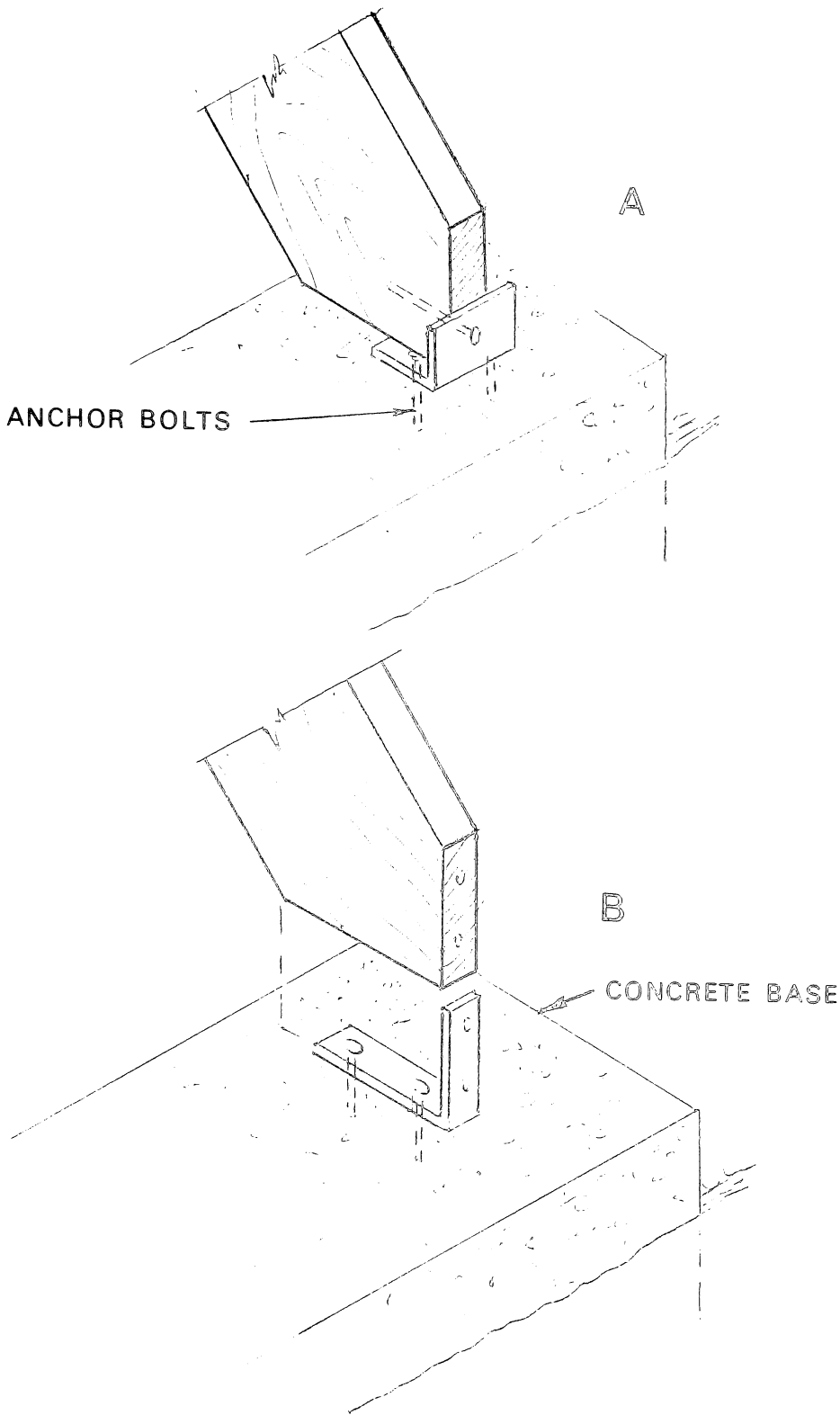
Figure 53. — Fastening the bottom of stair stringer. A and B — angle iron anchors.
