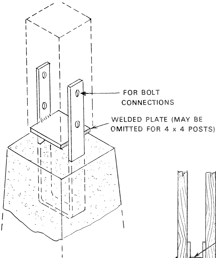
Figure 19. — Strap anchor.
