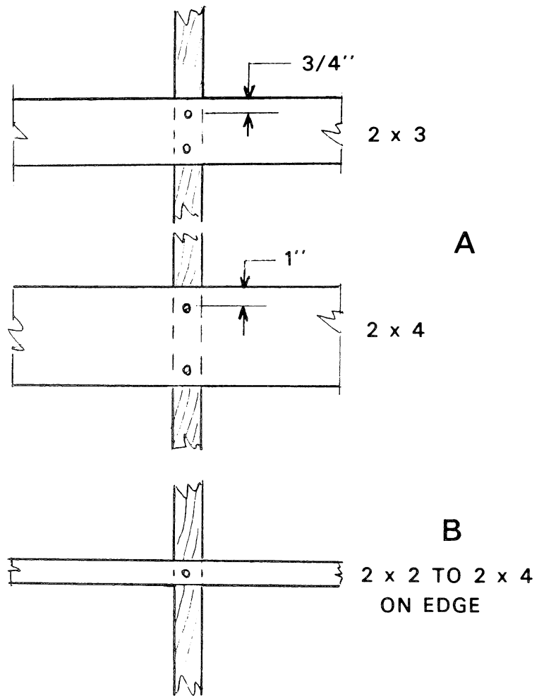
Figure 37. — Fastening deck boards. A — flat deck boards; B — deck boards on edge.
