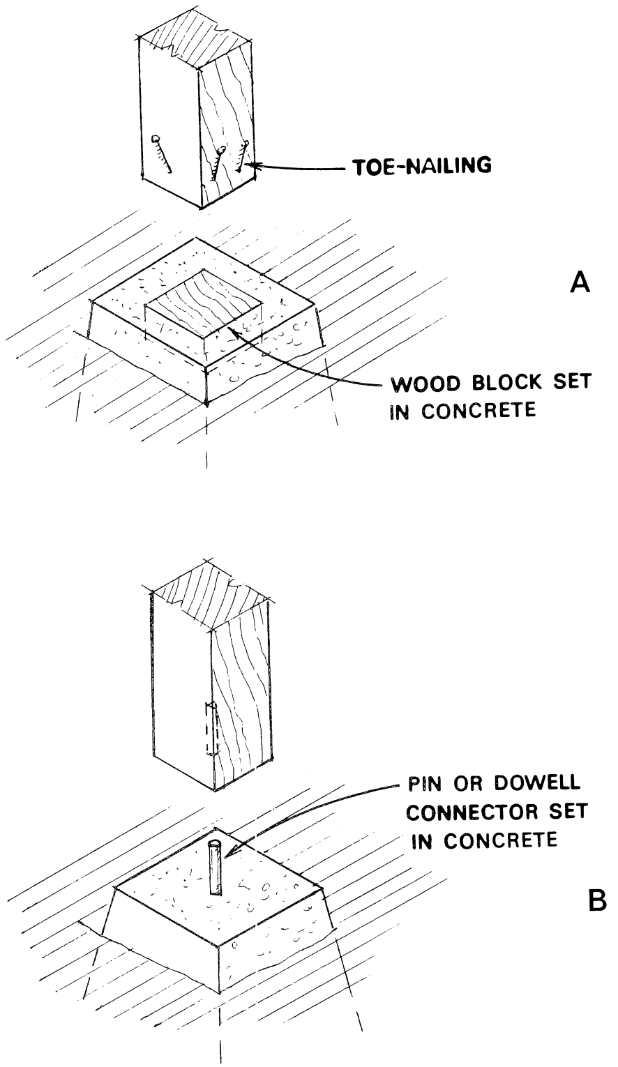
Figure 15. — Post-to-footing anchorage. A and B — poor practice.
