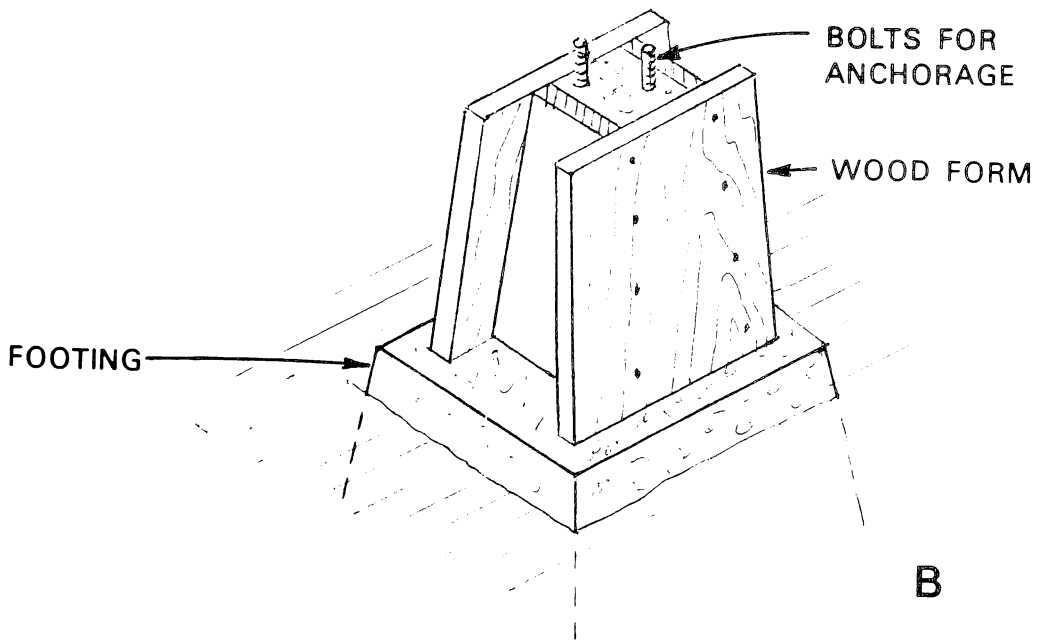
Figure 14. — Pedestal footing extension. A — pedestal for post; B — form used for pouring.
