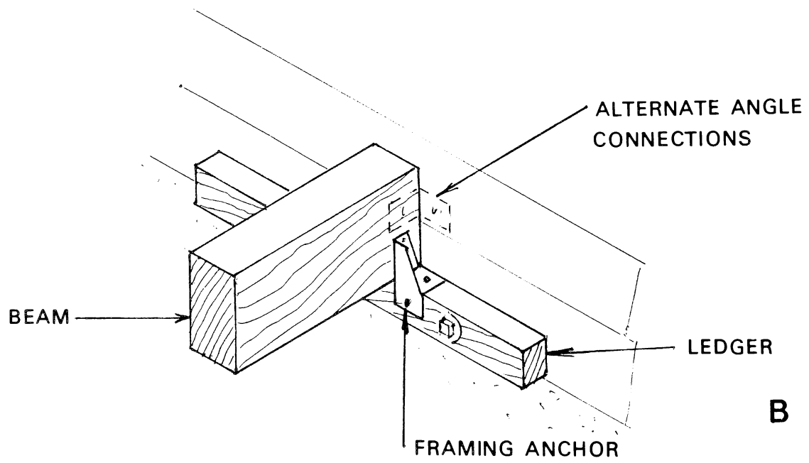
Figure 27. — Beam to house. A — beam hanger; B — ledger support.
