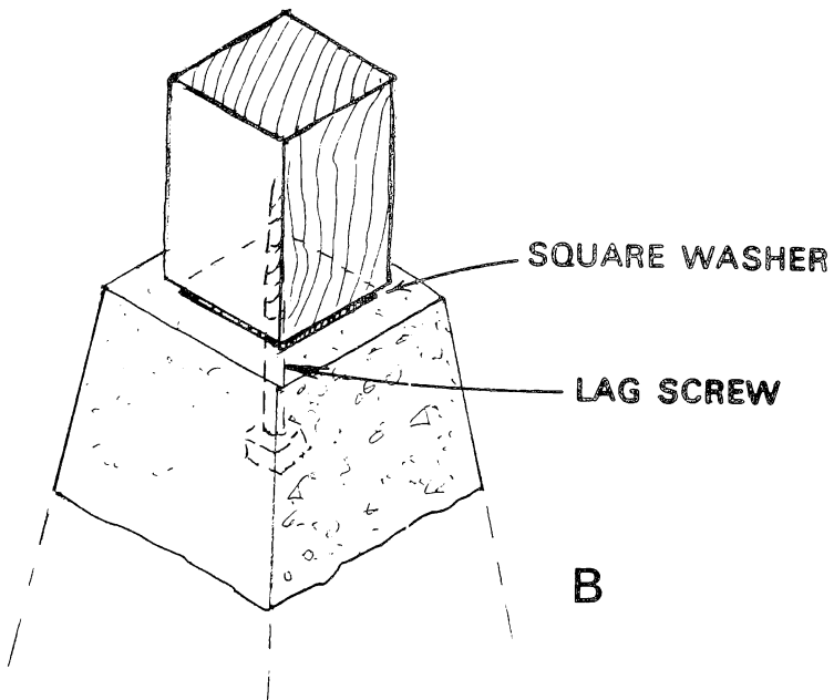
Figure 16. — Post-to-footing anchorage. A and B — improved practice.
