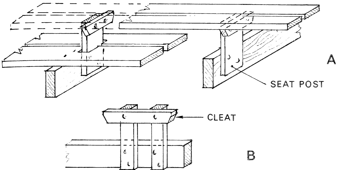
Figure 45. — Bench seats. A — single support and cross cleat; B — double support.
