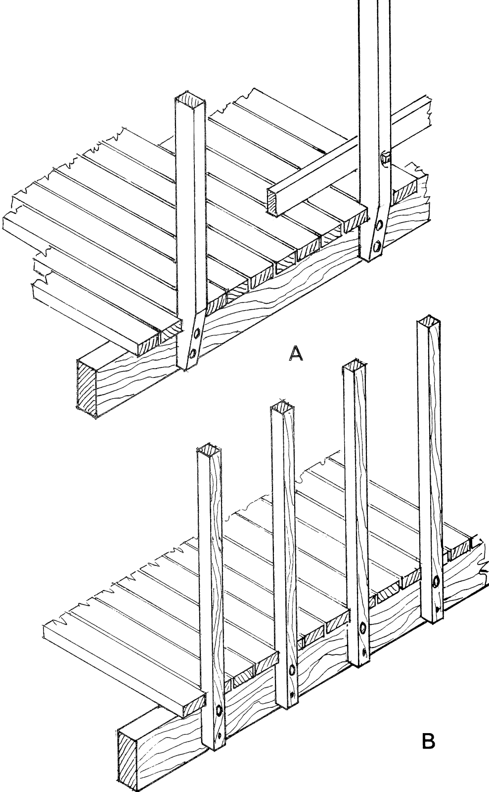
Figure 42. — Railing posts fastened to edge of deck member. A — spaced posts (4 feet and over); B — baluster-type posts.
