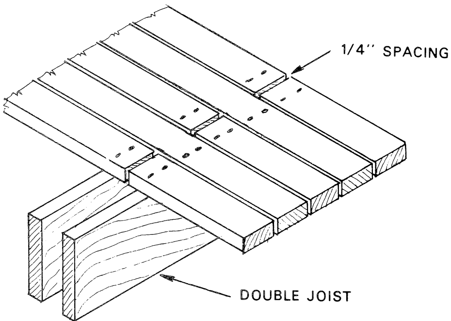
Figure 40. — End joints of decking over double joist.
