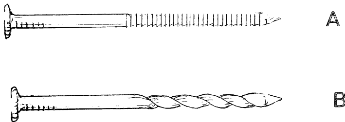
Figure 6. — Deformed shank nails. A — annular grooved (ring shank); B — spirally grooved.
