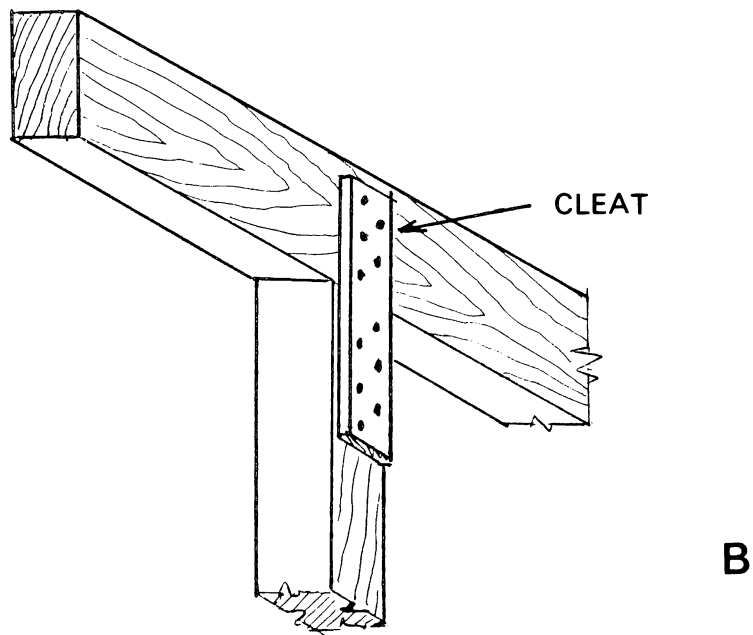
Figure 21.—Beam-to-post connection. A— toe-nailing, a poor practice ; B— better practice is to use cleat.
