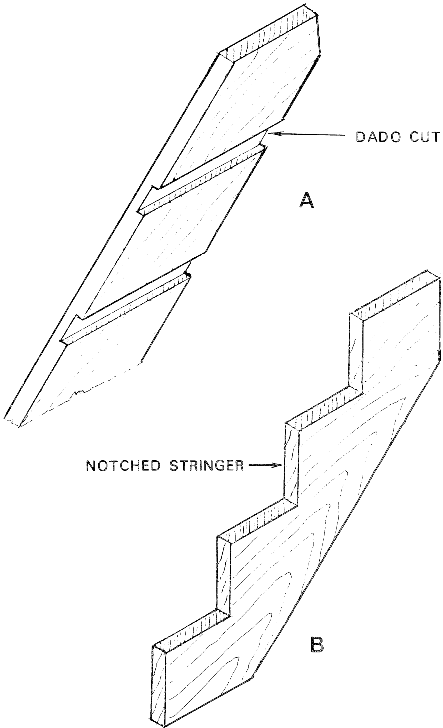
Figure 55. — Tread supports (not recommended). A — dadoed stringer (poor practice); B — notched (better practice).
