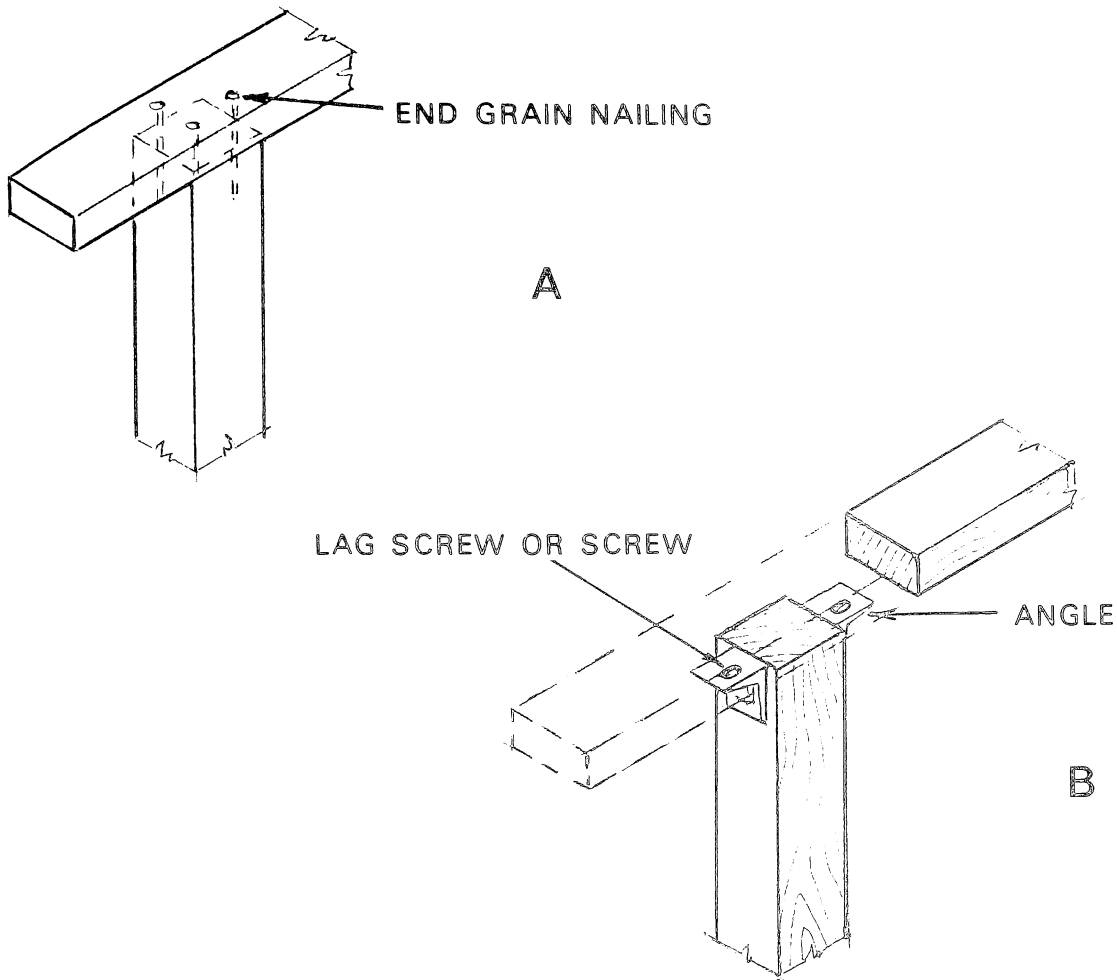
Figure 50. — Fastening cap rail to post. A — nailed (end grain), a poor practice; B — angle iron connection, a good practice.
