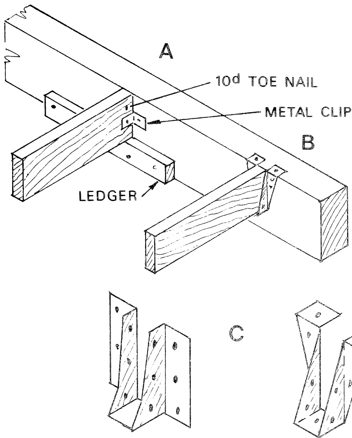
Figure 36. — Joists between beams. A — ledger support; B — joist hanger support; C — joist hangers.
