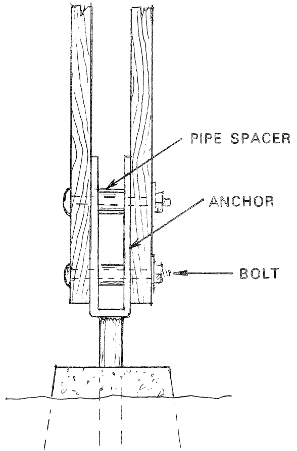
Figure 20. — Double post anchor (without bearing plate).
