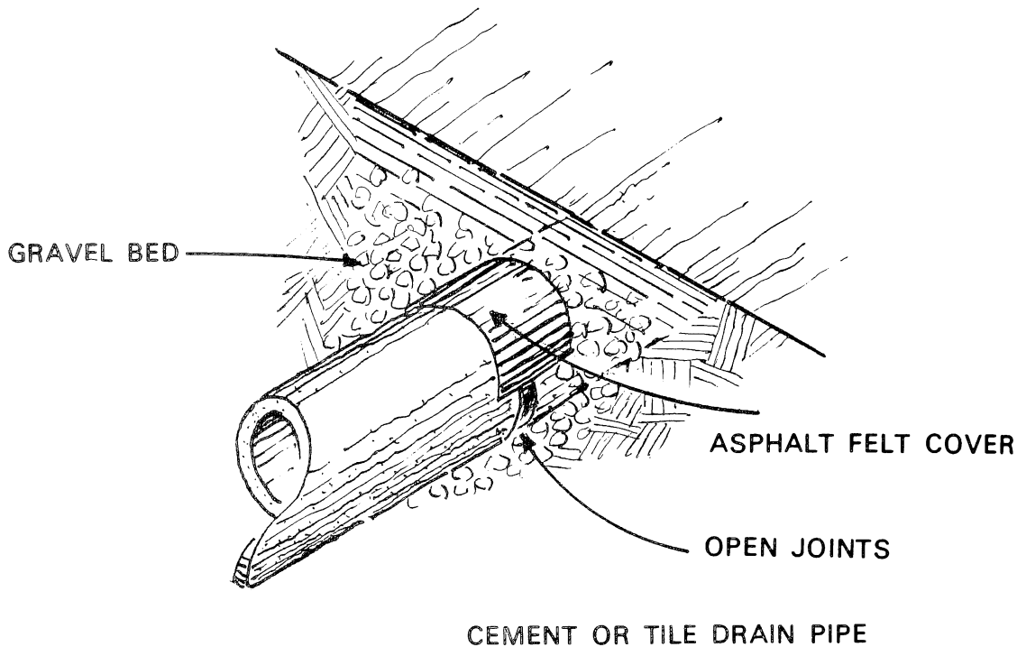
Figure 10. — Drain tile.
