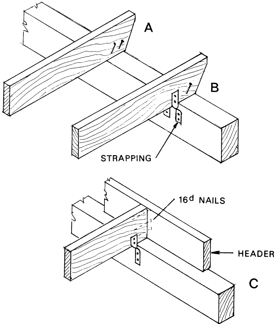
Figure 35. — Joist-to-beam connection. A — toe nail; B — strapping; C — connection with header.
