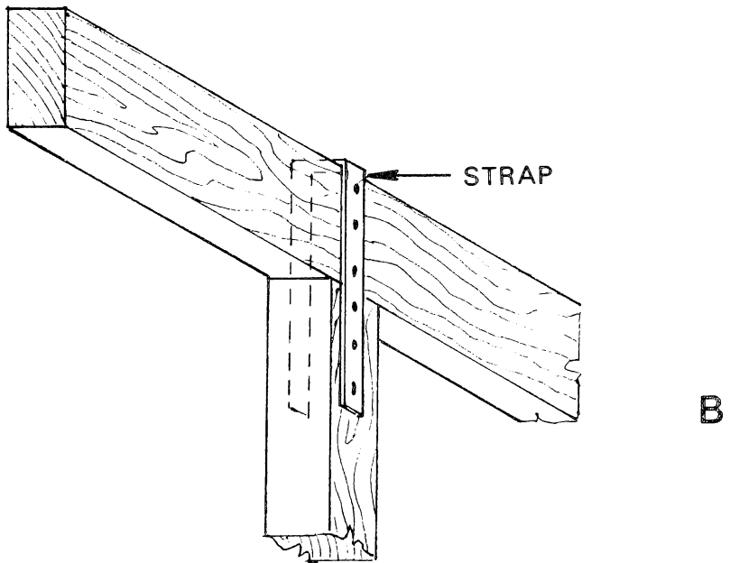
Figure 22. — Beam-to-post connection. Both A, angle iron, and B, strapping, are good methods.
