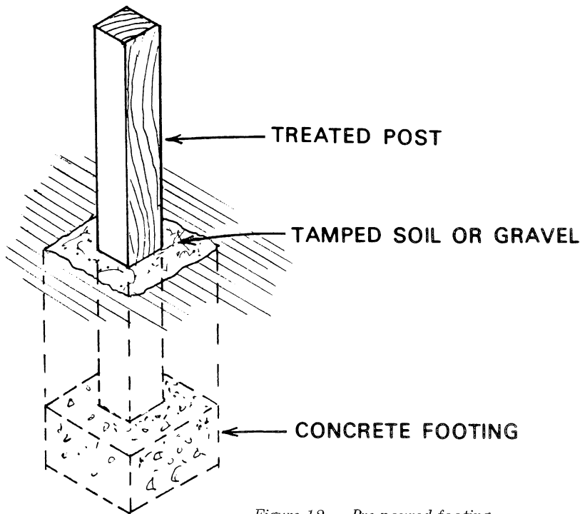
Figure 12. — Pre-poured footing.
