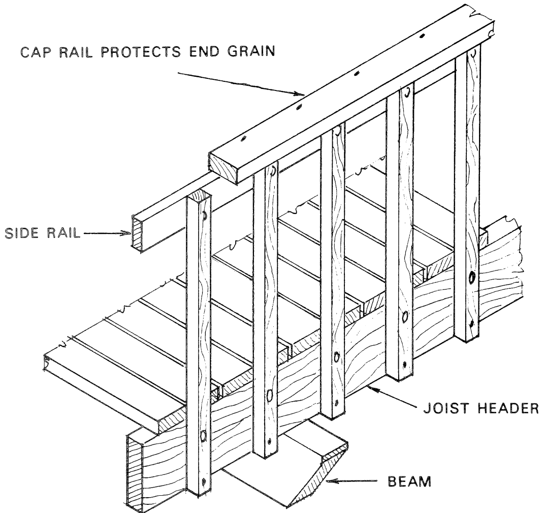
Figure 47. — Good railing detail.
