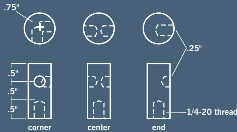
Stainless Steel Turret Post
