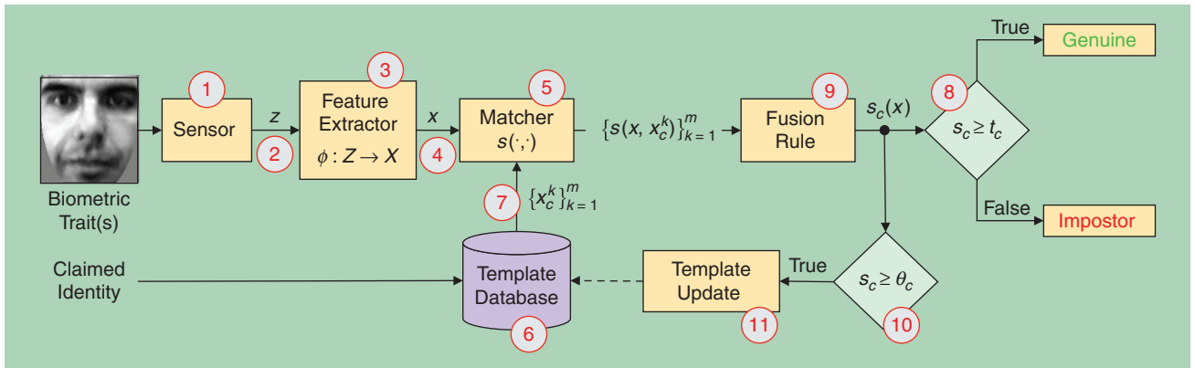
[FIG1] The architecture of a biometric verification system and corresponding attack points, highlighted with red-circled numbers. During verification, the image z \in \mathcal{Z} (e.g., a face image) acquired by the sensor is processed by a feature extractor \phi: \mathcal{Z} \rightarrow \mathcal{X} to obtain a compact representation x \in \mathcal{X} (e.g., a graph). The templates \{x_c^k\}_{k=1}^m of the claimed identity c are retrieved from the template database, and compared to x using a matching algorithm s: \mathcal{X} \times \mathcal{X} \rightarrow \mathbb{R} . The resulting scores \{s(x, x_c^k)\}_{k=1}^m are combined by a fusion rule, producing an aggregated score s_c(x) that expresses the degree to which x is likely to belong to c . The score s_c(x) is then compared with a decision threshold t_c to decide whether the claim is genuine or impostor. If a template self-update is implemented, and s_c(x) is not lower than a self-update threshold \theta_c , one of the templates in \{x_c^k\}_{k=1}^m is updated depending on x , according to a given policy.
