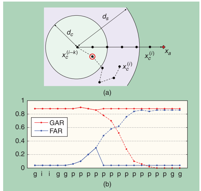
[FIG5] (a) Template sanitization. If the current centroid x_c^{(i)} falls outside the sanitization hypersphere (dark gray area), as for the poisoning attack sequence (solid line), the centroid x_c^{(i-k)} is restored; otherwise, as for the hypothesized genuine update sequence (dashed line), the center of the sanitization hypersphere is updated to x_c^{(i-k+1)} (red circled point). (b) GAR and FAR values in the presence (solid lines) and in the absence (dashed lines) of template sanitization, after different centroid updates, including genuine ("g") and impostor ("i") attempts, and poisoning attacks ("p") with perfect knowledge.
