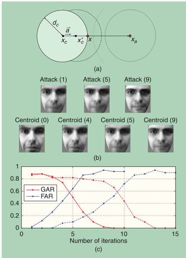
[FIG4] (a) A poisoning attack with perfect knowledge. The circles centered on x_a represent the objective function \|x - x_a\| , minimized by the attack point x on the feasible domain \|x - x_c\| \leq d_c . The updated centroid x'_c and the feasible domain for the next attack iteration are also shown. (b) Attack samples and the victim's centroids for poisoning with perfect knowledge at different iterations. (c) Genuine acceptance rate (GAR) and false acceptance rate (FAR) values in the presence (solid lines) and in the absence (dashed lines) of template sanitization, after different centroid updates, including genuine ("g") and impostor ("i") attempts, and poisoning attacks ("p") with perfect knowledge.
