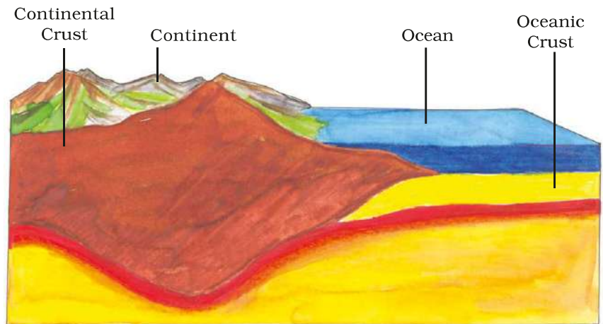
Fig. 2.2: Continental Crust and Oceanic Crust
