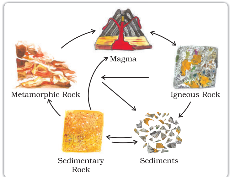
Fig. 2.4: Rock Cycle
