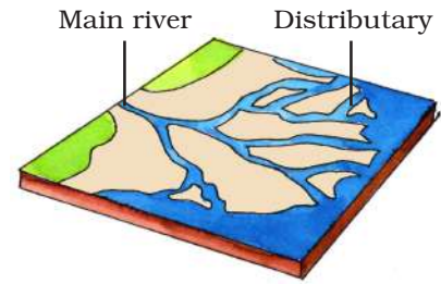
Fig. 3.6: A Delta
