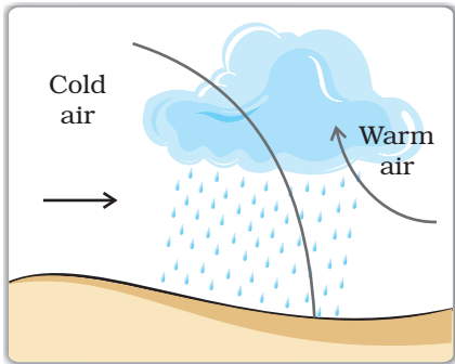
Cyclonic Rainfall
