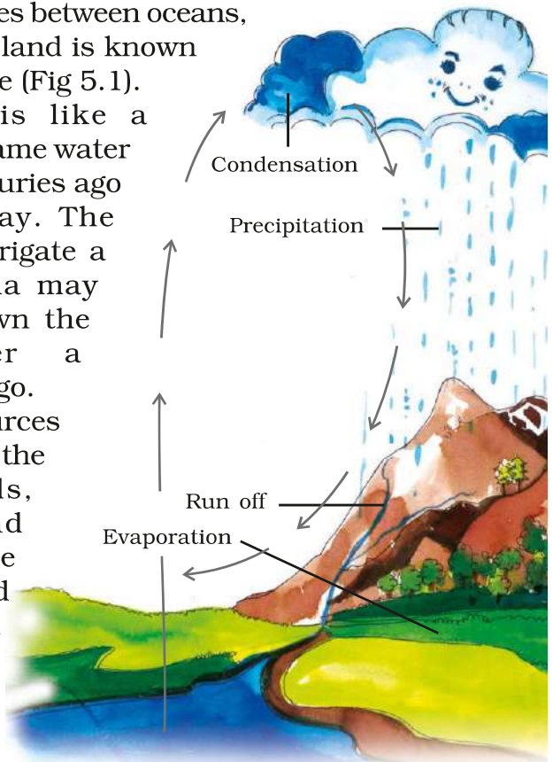
Fig. 5.1: Water Cycle
