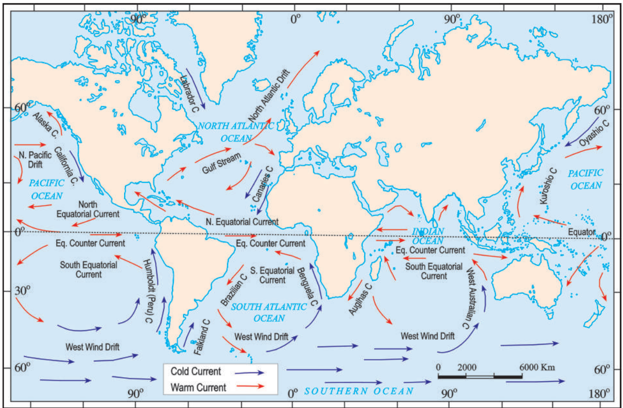
Fig. 5.6: Ocean Currents
