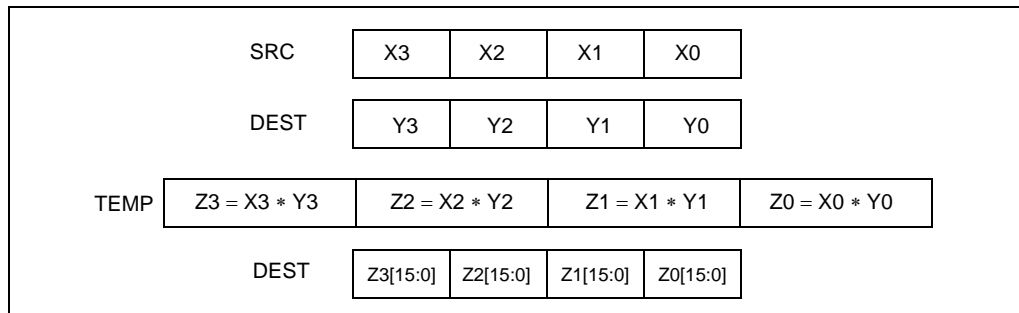
Figure 4-4. PMULLW Instruction Operation Using 64-bit Operands
