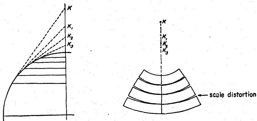
FIG. 48.—Polyconic development.
