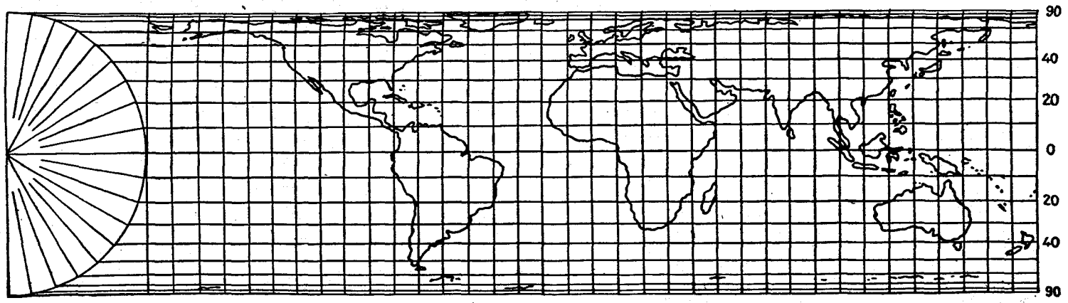
FIG. 16.—Cylindrical equal-area projection.
