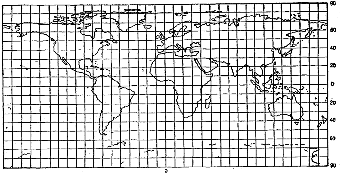
FIG. 17.—Cylindrical equal-spaced projection.
