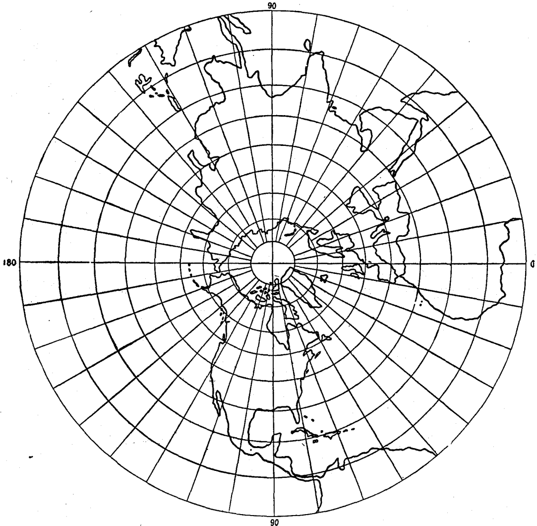
FIG. 22.—Stereographic polar projection.
