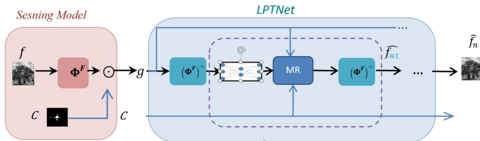
Fig. 24 Schematic description of the learned compressive Fresnel holography: LPTnet is used to determine the hologram sampling point and the parameters of the reconstruction deep neural network
