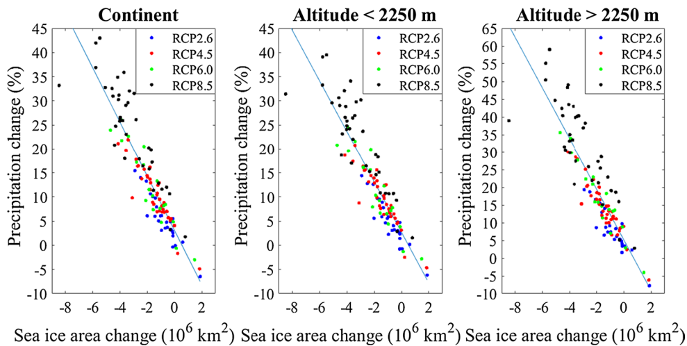
Fig. 9 Antarctic precipitation and annual-mean sea ice area in the southern hemisphere changes between the periods 1986–2005 in the Historical scenario and 2080–2099 in the four RCP scenarios
