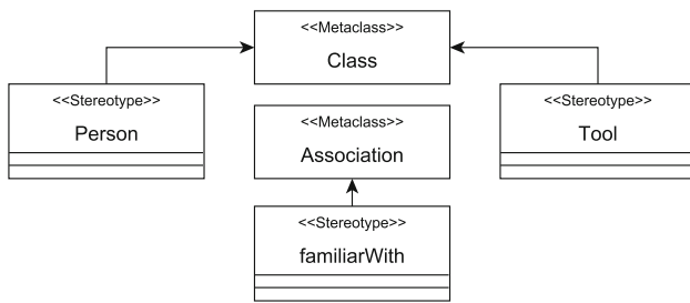
Fig. 5 Example UML profile for SDPL showing Person, Tool and the familiarWith association
