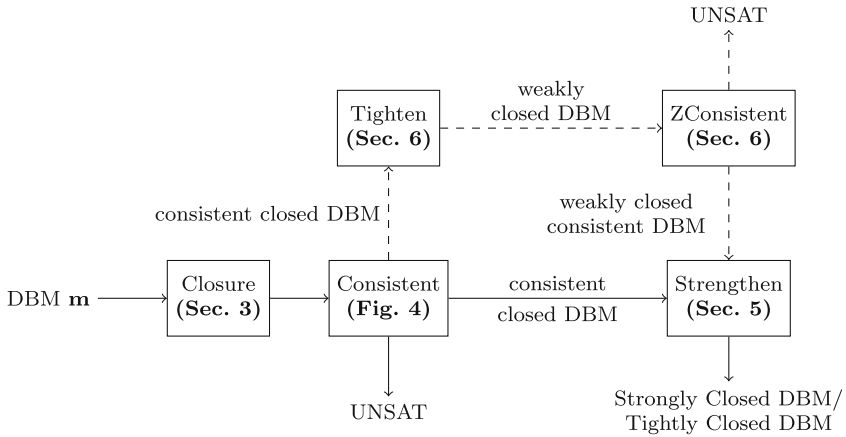
Fig. 3 High-level overview of closure algorithms for octagons
