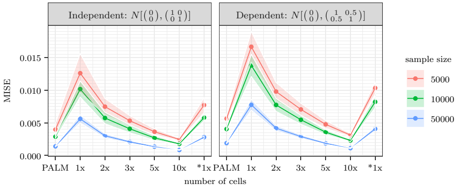
Fig. 8 For data generated from a two-dimensional Gaussian distribution, described in Sect. 7.4, the mean and standard deviation of MISE is calculated for different partitions: (from left to right) PALM, fixed grid with the same number of regions as PALM (denoted as ‘1x’), fixed grid with two times number of regions as PALM (denoted as ‘2x’), ..., and fixed grid with the same number of regions before the merging step of PALM (denoted as ‘*1x’). We assume S = [-5, 5] \times [-5, 5] , as the true Gaussian density outside S is negligible
