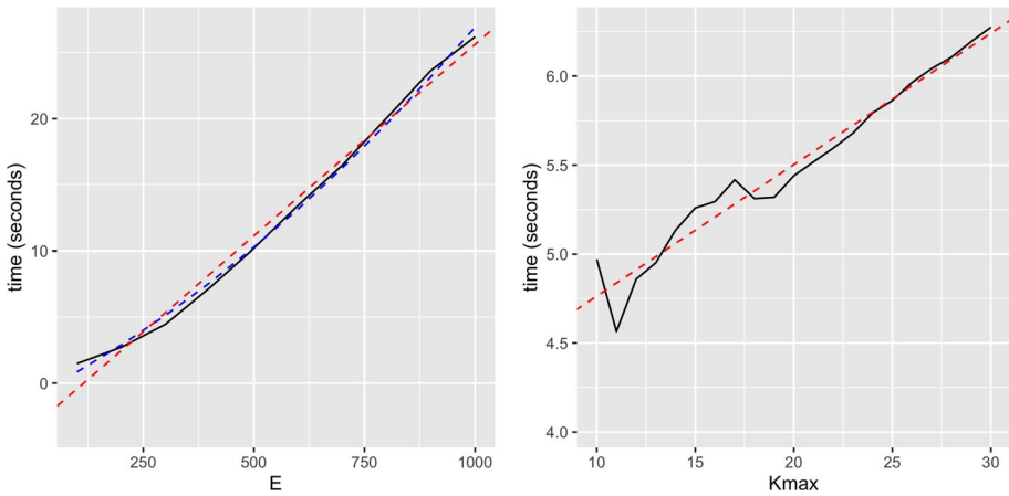
Fig. 10 Empirical time complexity on simulated two-dimensional Gaussian data, with respect to E , the number of candidate cut points, and the runtime, and K_{max} , the maximum number of bins we search
