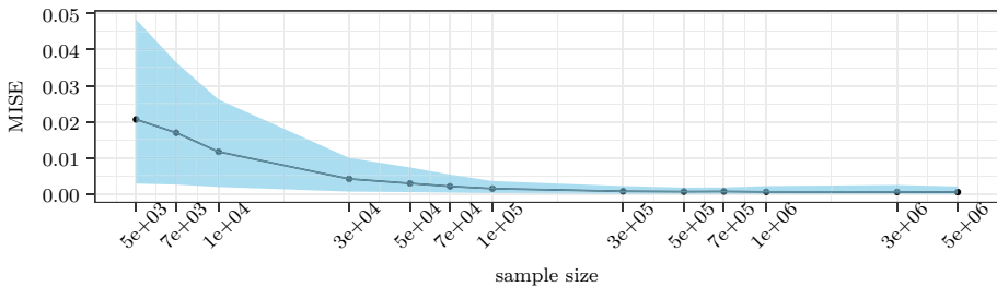
Fig. 4 Sample size versus MISE: MISE converges to almost 0 when the sample size becomes larger than 100,000. The range between the 5th and 95th percentiles is shown in blue
