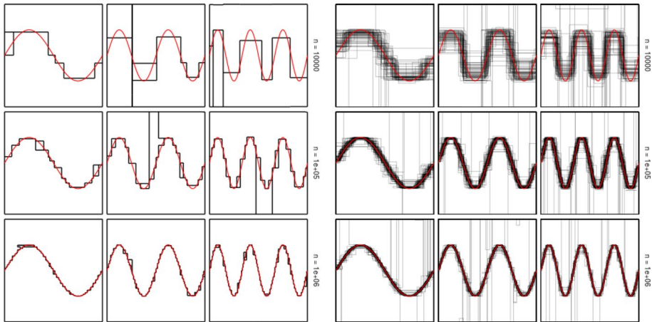
Fig. 6 (Left) Sine curve defined in Eq. (27) (red), with m \in \{2, 4, 6\} from left to right on each row, and the learned partition by PALM (black). Data is randomly generated by uniform distribution above and below the sine curve, within S = [0, 1] \times [0, 1] . Densities above and below the sine curve are 2:1. From top to bottom, the sample sizes of the simulated data are n \in \{1e4, 1e5, 1e6\} . (Right) 50 partition results of 50 different simulated datasets are plotted together. It shows that PALM is not guaranteed to be absolutely stable, as it occasionally produces undesired extra line segments, but the line segments of the learned partitions mostly gather around the true sine curve
