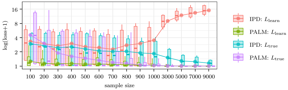
Fig. 9 Comparison of PALM and IPD, using the box-plot and the mean of L_{learn} and L_{true} , as defined in Eq. (24). PALM not only performs better when the sample size is small, but also converges as the sample size increases, while IPD does not converge
