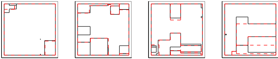
Fig. 3 Random examples of true (black solid) and learned partitions (red dashed) of the experiment in Sect. 7.2, mainly to show that our experiment settings can produce very flexible partitions of [0, 1] \times [0, 1] . Note that the sample size is set as 10 000, which is not enough for MISE (Equation 23) to converge to almost 0, but the learned partitions by PALM already look promising: it can partly identify the true partitions
