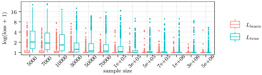
Fig. 5 Boxplots showing the sample size versus L_{\text{learn}} and L_{\text{true}} as defined in Eq. (24). Note that the y-axis has a logarithmic scale. L_{\text{learn}} is generally much smaller than L_{\text{true}} , meaning that it is very rare that PALM produces unnecessary extra regions. When the sample size is large enough for MISE to converge ( n \geq 1e5 ), outliers of L_{\text{true}} are due to sampling variance when generating the true parameters f_j defined in Equation (26), see Table 1; the number of outliers for L_{\text{learn}} decreases rapidly as the sample size becomes larger, as they are due to sampling variance when generating the data
