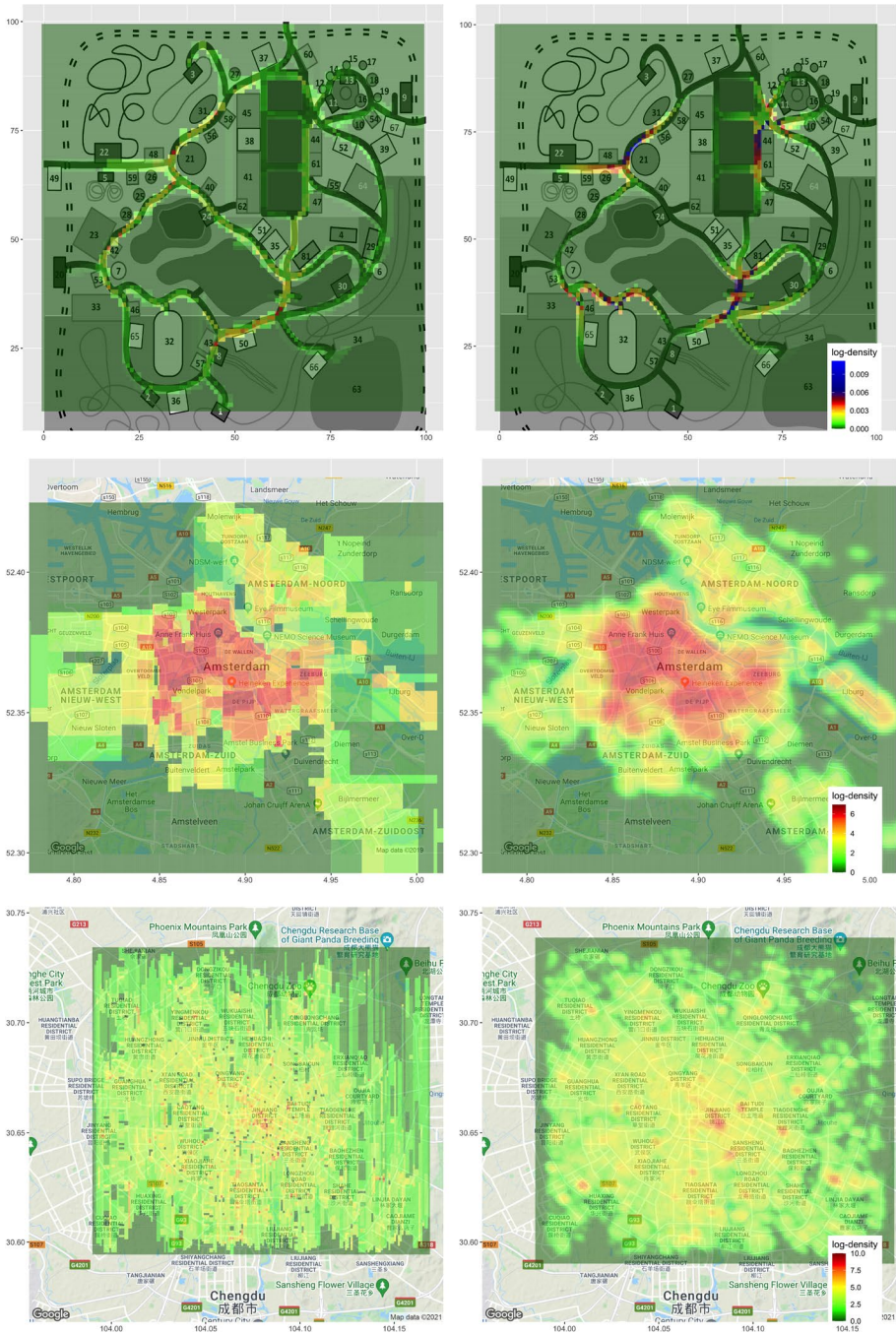
Fig. 11 Estimated densities on three real-world datasets using PALM (left) and KDE (right); from top to bottom: DinoFun amusement park, Amsterdam Airbnb housing, and taxi destinations in Chengdu
