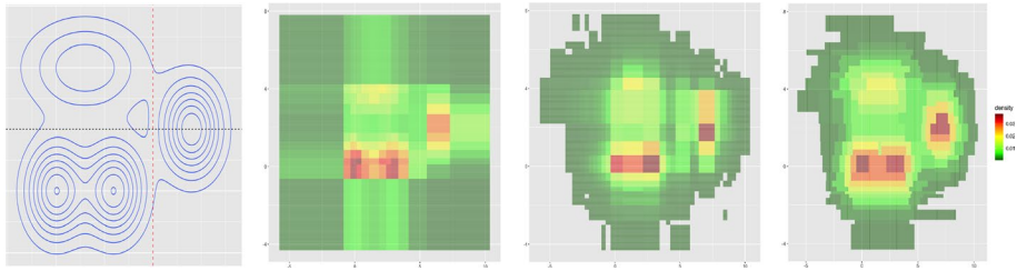
Fig. 1 Distributions of a two-dimensional dataset simulated from a mixture of Gaussian distributions; from left to right: (1) true probability density contour, (2) partitioning by IPD (Nguyen et al., 2014), (3) partitioning by separately discretizing each dimension with the MDL histogram (Kontkanen & Myllymäki, 2007), (4) flexible partitioning by PALM, our algorithm
