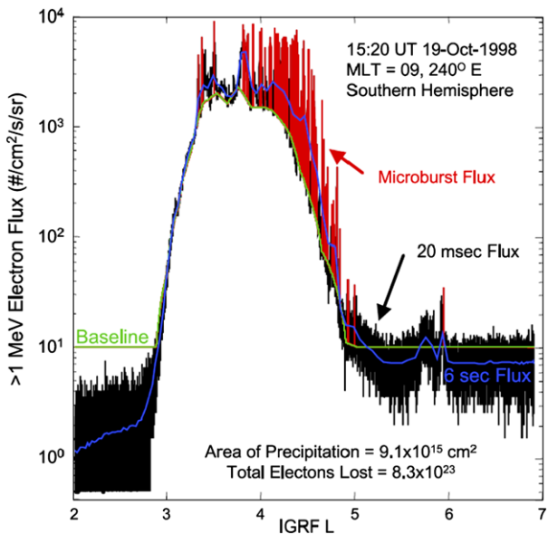
Fig. 14 SAMPEX observations of so-called microburst precipitation of relativistic electrons into the belts with transient time scales of <20 milliseconds. From O’Brien et al. (2004). © The American Geophysical Union
