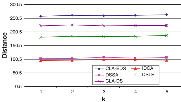
Fig. 10 Comparison of CLA-EDS with existing deployment algorithms in terms of the distance criterion for N = 1,500 sensor nodes
