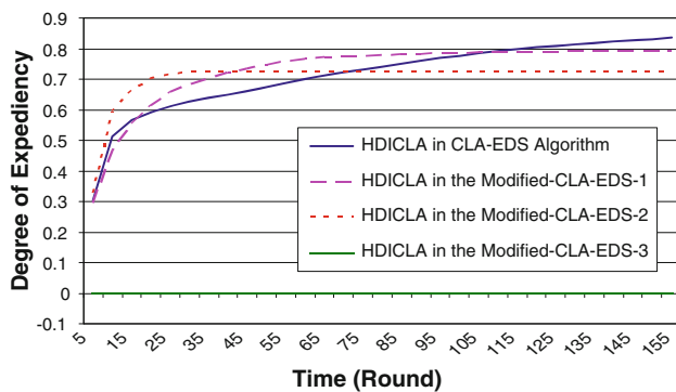
Fig. 31 Degree of expediency of the HDICLA
