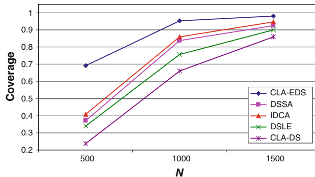
Fig. 23 Comparison of CLA-EDS with existing deployment algorithms in terms of the coverage criterion when the required degree of coverage differs in different regions of the network
